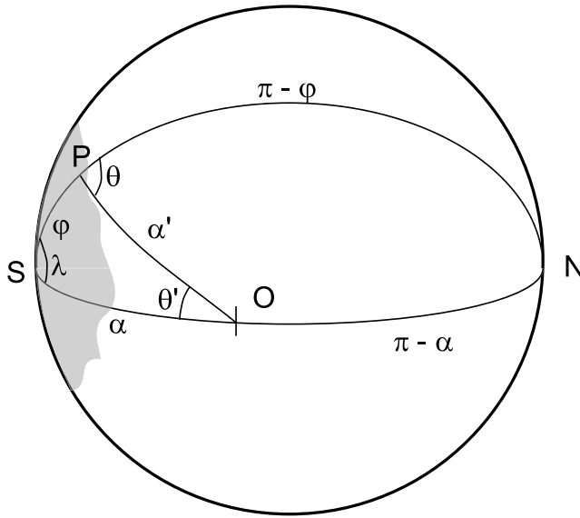
Figure 7. Geometry of the “fossil” swell field distribution at time t_0 = 0 (shaded area) and observation conditions. Any point P of colatitude \varphi and longitude \lambda inside of the storm generates waves that are observed at point O . At time t the observed waves that come from P have a well-defined frequency given by equation (C2), the function of the spherical distance \alpha' between P and O , and a well-defined direction \theta at P relative to the north, which gives a direction \pi - \theta' at O . In the triangle OPS the angles \lambda , \theta' , and \pi - \theta are related to the distances \alpha' , \varphi , and \alpha by the usual spherical trigonometry relationships, e.g., equation (C4).
