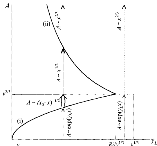
FIGURE 6. The amplitude-supercriticality diagram for a slightly stratified flow when Ri \ll v^{2/3} , Pr > 1 . (i) A \sim (\gamma_L v^{5/3}/Ri)^{1/2} ; (ii) A \sim (Ri/\gamma_L)^2 ; the arrows indicate the different evolutionary stages.
