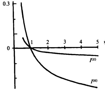
FIGURE 3. Evaluation of the integral in (4.20): I^{(2)} = (1-\eta) a_0^2(\eta) ; I^{(0)} = (1-\eta) a_0^{(0)}(\eta) .
