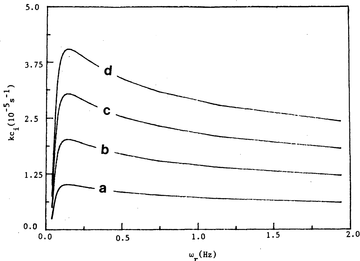
FIG. 4. As in Fig. 3 except for 2h = 5 m. Note also that the ordinate has a different scale.
