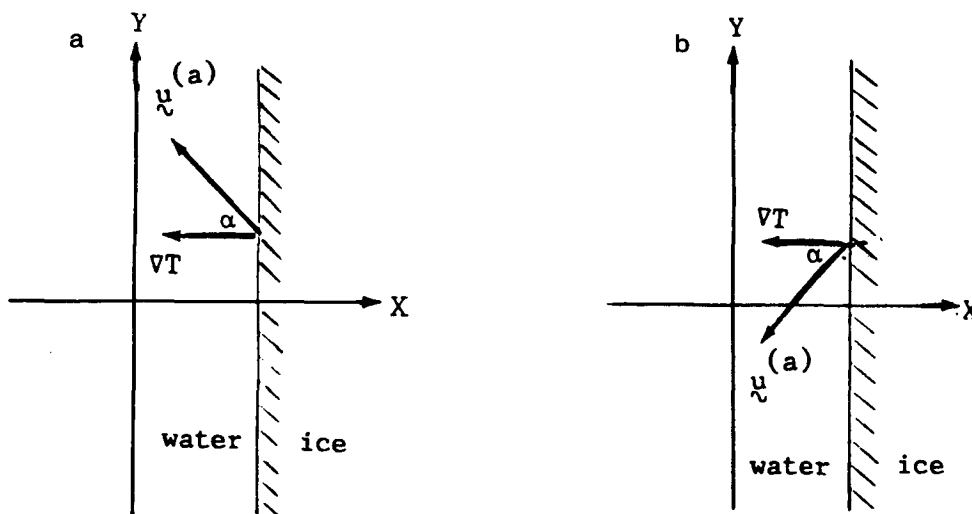
FIG. 2. Thermally forced wind near ice edge. (a) North polar region; (b) South polar region.
