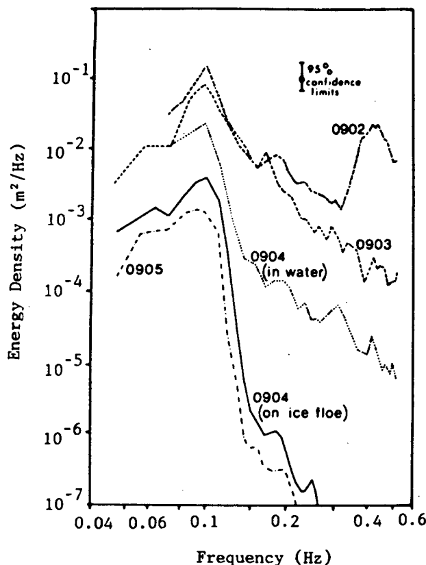
FIG. 6. Observed energy density spectra of ocean wave entering an ice field (from Wadhams et al., 1986).
