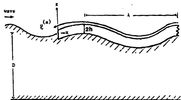
FIG. 1. An air-ice-ocean coupled system.
