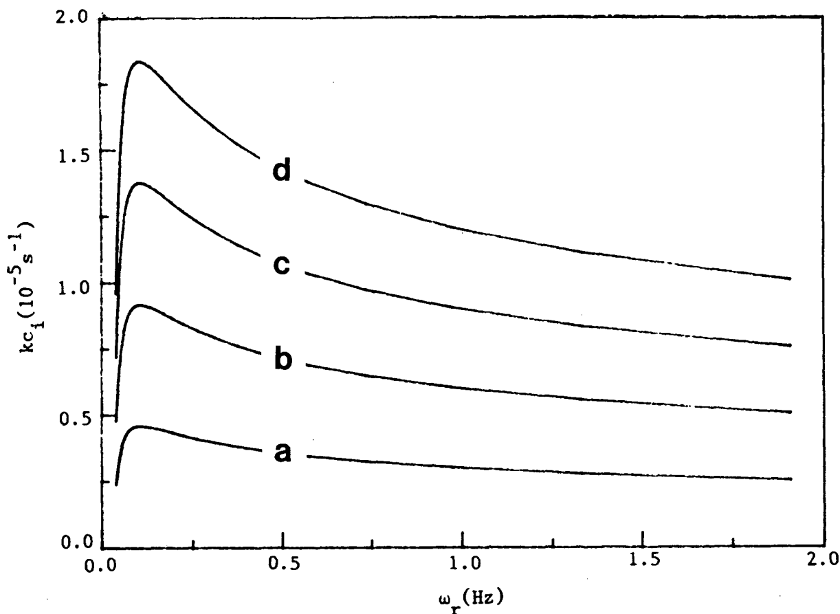
FIG. 5. As in Fig. 3 except for 2h = 10 m. Note also that the ordinate has a different scale.
