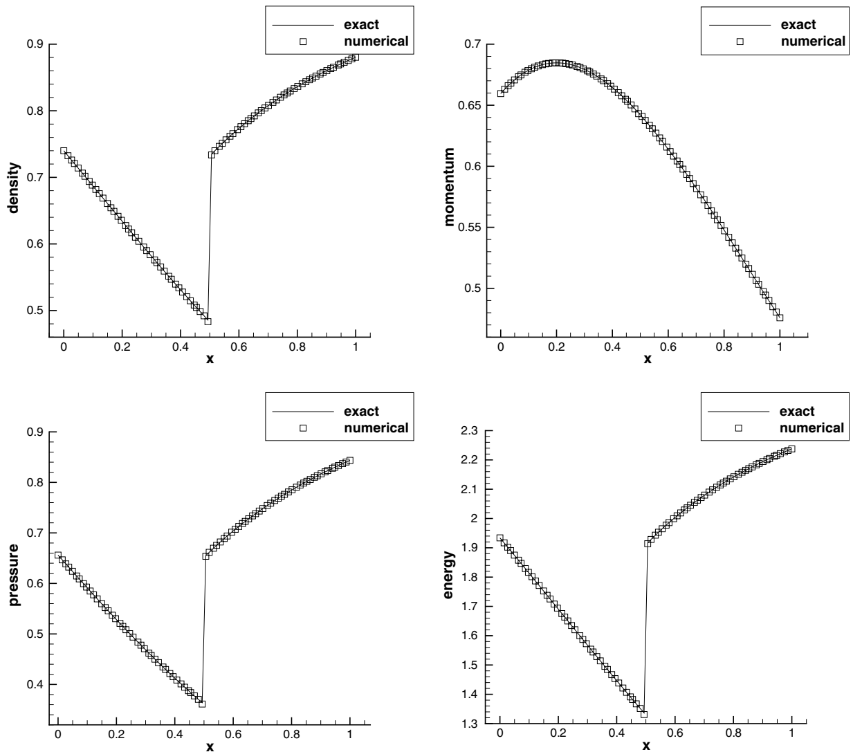
Fig. 3. Nozzle flow problem. Non-smooth mesh with 81 cells. Solid lines: exact solution; symbols: numerical solution. Top left: density; top right: momentum; bottom left: pressure; bottom right: total energy.
