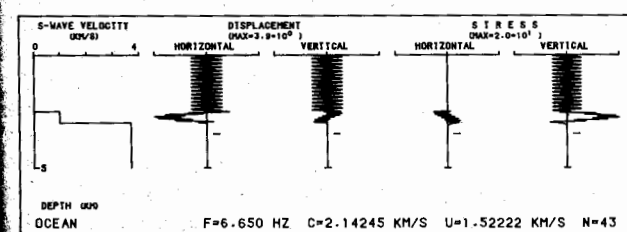
Fig. 6a-d. Eigenfunctions of the oceanic model. a, b, c and d correspond respectively to points 4, 5, 6 and 7 in Fig. 5a. Symbols in the plot are as for Fig. 2
