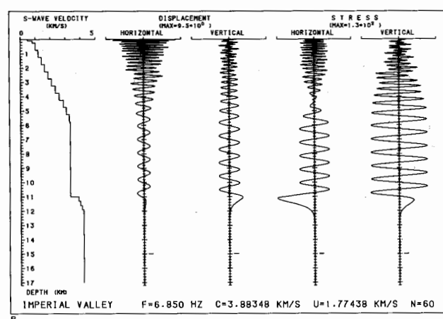
Fig. 8a and b. Eigenfunctions of the continental model IMP1. a sedimentary wave, b upper crustal wave. Symbols in the plot are as for Fig. 2
