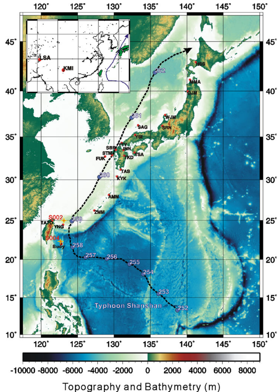
Fig. 1 Regional bathymetry and station location map with the track of Typhoon Shanshan. (Blue dots depict the beginning of the Julian day). Buoy marks the location of Taitung deep sea weather buoy. S002 and S004 mark the locations of the two ocean bottom seismometers. All other stations are land stations, mostly from F-net of Japan. Typhoon Shanshan moved alongside this 2,000-km seismic array, exciting interesting ground motions analyzed in this study. Stations KMI and LSA are part of the Global Seismic Network (GSN; see inset )
