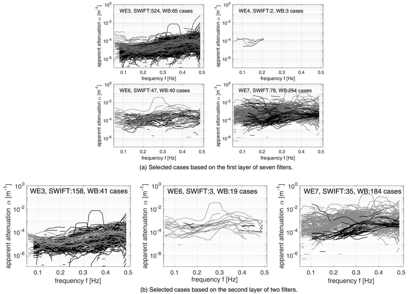
Figure 4. Collection of the apparent attenuation coefficient \alpha in WE3, 4, 6, 7 based, (black – SWIFT, grey – WB). (a) Selected cases based on the first layer of seven filters. (b) Selected cases based on the second layer of two filters.
