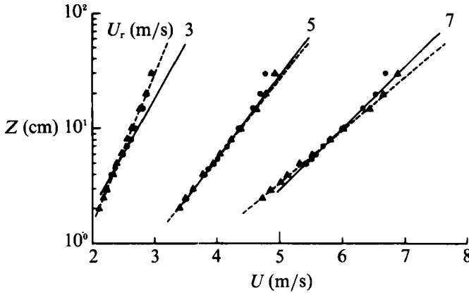
FIGURE 3. Wind profiles over the water surface for pure wind-waves and the co-existing system of wind-waves and the swell propagating in the direction of the wind. H_0/L : \blacktriangle , 0 (pure wind-waves); \bullet , 0.04.
