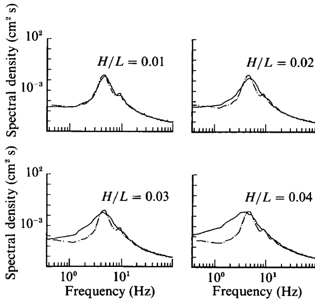
FIGURE 7. Power spectra of the pure wind-waves and wind-waves affected by the opposing swell. U_r = 5 m/s and F = 8 m. ---, the pure wind-waves; —, wind-waves affected by the opposing swell. Swell steepness H_0/L : 0.01, 0.02, 0.03 and 0.04.
