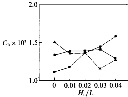
FIGURE 5. The drag coefficient C_D (= (u_*/U_{10})^2) versus the swell steepness H_0/L for the co-existing system of wind-waves and the swell propagating in the direction of the wind. U_r (m/s): ●, 3; ■, 5; ▲, 7.
