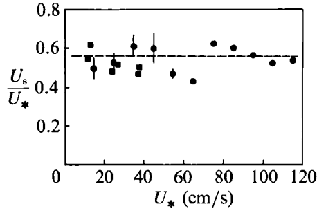
FIGURE 10. The dimensionless surface drift velocity U_s/U_* versus the wind friction velocity U_* for the pure wind-waves. \bullet , \bullet , Wu (1973); \blacksquare , the present data; ---, U_s/U_* = 0.55 .
