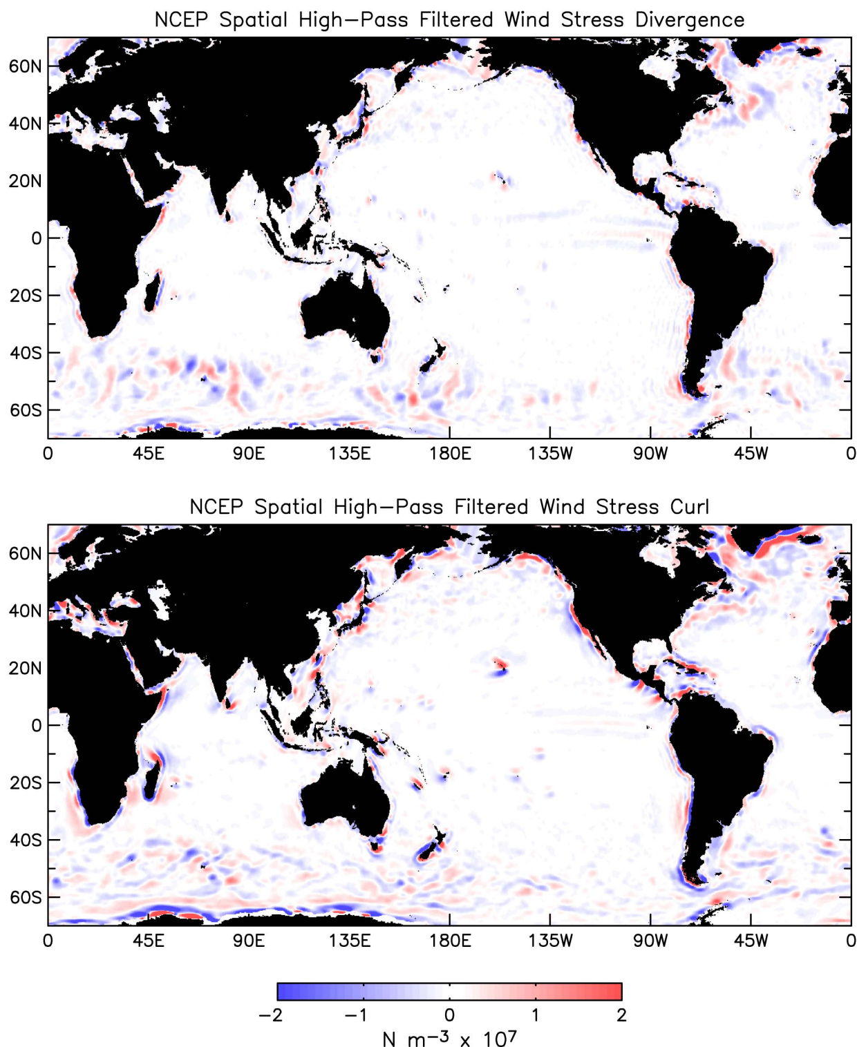
Fig. S3. The same as Fig. S2, except computed from the 1° by 1° by 6-hour analyses of winds at 10 m from the U.S. National Centers for Environmental Prediction (NCEP) operational numerical weather prediction model. Some of the small-scale features in the QuikSCAT divergence and curl fields are also evident in the NCEP fields, but generally with smaller amplitudes and larger scales. The alternating bands of positive and negative divergence and curl near many of the continental boundaries (especially evident off the west coasts) are artifacts of spectral truncation of mountain topography in the spherical harmonic NCEP model (S1).
