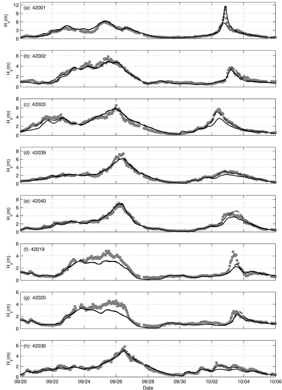
FIG. 3. Time series of H_s (m) at selected NOAA/NDBC buoy locations. Lines and markers are as in Fig. 2.
