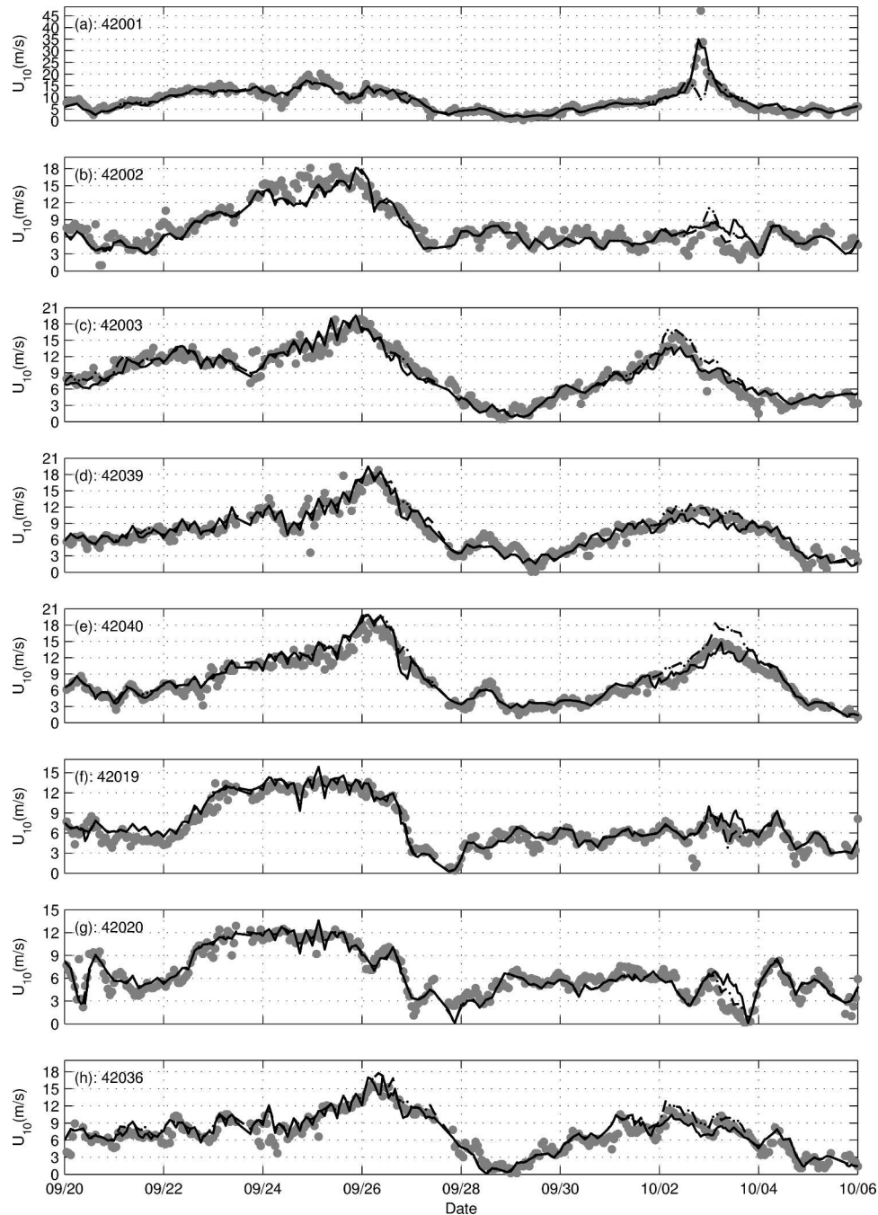
FIG. 2. Time series of U_{10} ( \text{m s}^{-1} ) at selected NOAA/NDBC buoy locations. Hindcast data from the WNA (dashed line) and NAH (solid line) models are compared to observations (gray circles).
