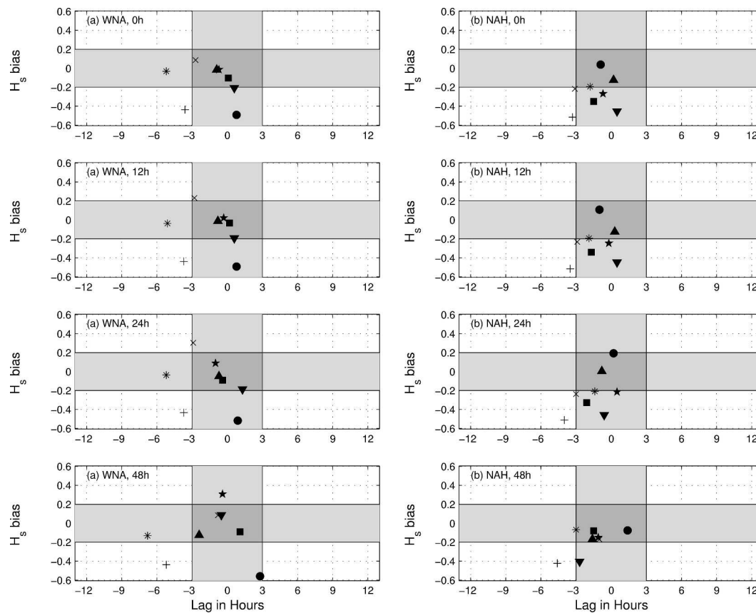
FIG. 11. Accuracy of the NAH model in predicting the maximum waves generated by Hurricane Lili at selected NDBC buoy locations. Buoy patterns: 42001 (filled circle, ●), 42003 (filled triangle, ▲), 42019 (plus sign, +), 42020 (asterisk, *), and 42036 (filled inverted triangle, ▼). See text for approach used for computing maximum H_s bias and time lag.
