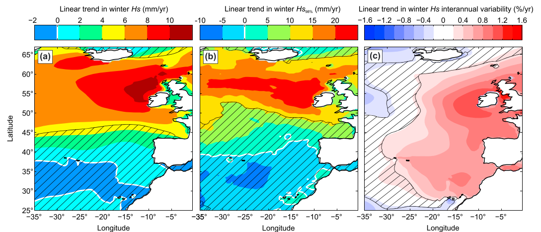
Figure 3. Linear trend of (a) winter-mean (1949–2017) H_s and (b) its 98% exceedance values H_{s98\%} in millimeter/year and of (c) winter-mean (1949–2017) H_s interannual variability in percent/year. The hatched zones are areas where trends and correlations are not significant at the 95% confidence level.
