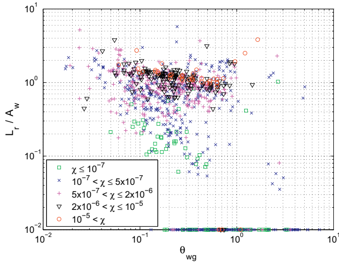
Fig. 2. Wave-generated ripple wavelength normalised by the wave orbital semi-excursion as a function of the grain-related Shields parameter with the wave period parameter emphasised.
