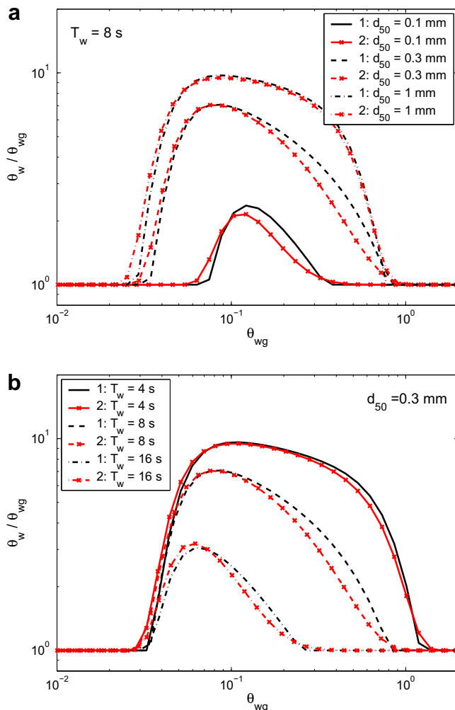
Fig. 9. Total Shields parameter versus the skin Shields for several median grain sizes (a) and wave periods (b) using the classical method based on the prediction of the ripple characteristics (1: black lines) or Eq. (19) (2: red lines with crosses) (for interpretation of the references to colour in this figure legend, the reader is referred to the web version of this article).
