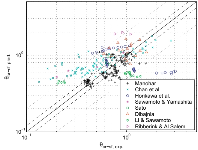
Fig. 1. Estimation of the critical Shields parameter for the inception of wave-related sheet flow using Eq. (8).
