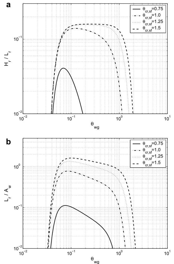
Fig. 4. Ripple steepness H_r/L_r (a) and ratio L_r/A_w (b) versus the skin Shields parameter for several values of the critical Shields parameter for the inception of sheet-flow \theta_{cr, sf} using Eqs. (9) and (10) with \alpha_{cr} = 1 and d_{50} = 0.3 mm.
