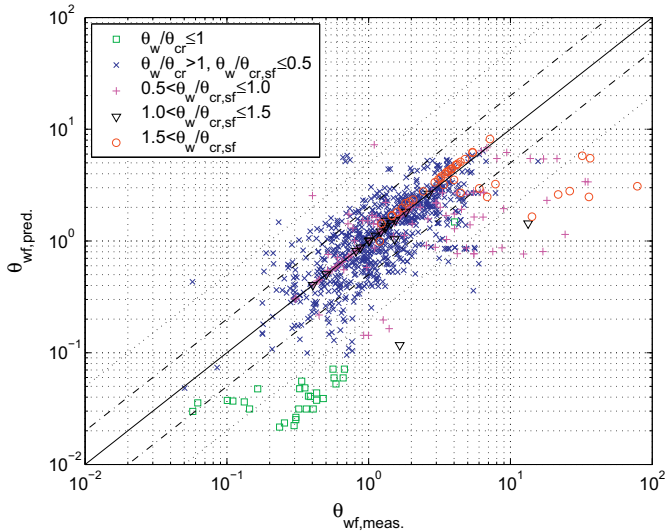
Fig. 10. Prediction of the Shields parameter using Eq. (17) with a_r = 20 for the estimation of the roughness and the observed and estimated (Eqs. (9) and (10) with a_{cr} = 1 ) characteristics of the ripples.
