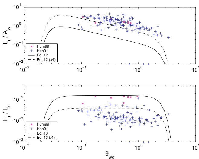
Fig. 5. Large wave ripple (LWR) wavelength (normalised by the wave orbital semi-excursion) and steepness as a function of the grain-related Shields parameter.
