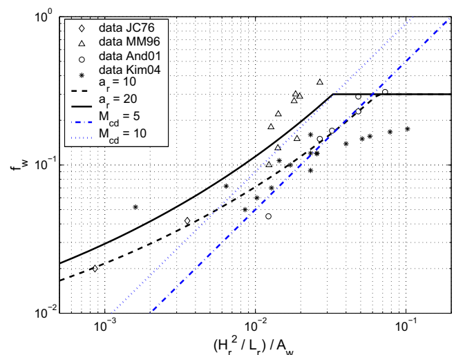
Fig. 8. Wave-related friction coefficient f_w as a function of (H_r^2/L_r)/A_w (Eq. (16) and Eq. (18) are plotted, using Eq. (17) with a_r = 10 and 20 , and M_{cd} = 5 and 10 , respectively, together with experimental data from Jonsson and Carlsen (1976) and Mathisen and Madsen (1996), and numerical data from Andersen (2001) and Kim (2004)).
