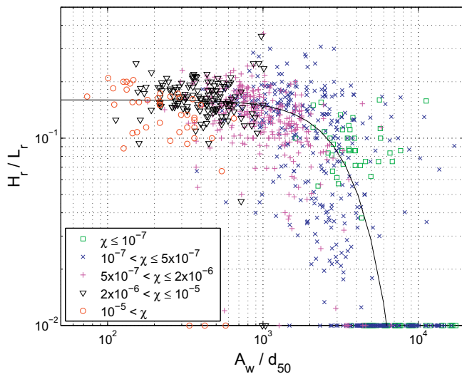
Fig. 3. Wave-generated ripple steepness as a function of the wave orbital semi-excursion normalised by the median grain size with the wave period parameter emphasised (the solid line corresponds to Eq. (13)).
