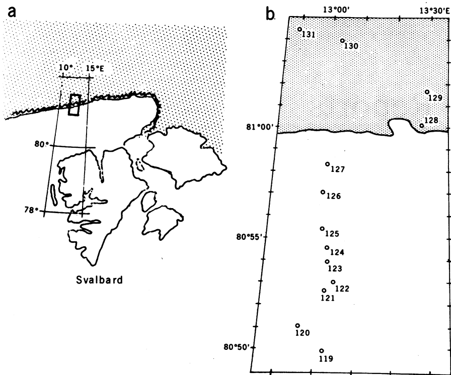
Fig. 1. (a) The location of the polar ice pack relative to Spitsbergen (called Svalbard in Norwegian) as drawn from a NOAA-5 satellite image taken in late November 1977. The shaded area represents the area covered by more than 6/8 pack ice. The small rectangle at about 81°N, 13°E is the area discussed in this report. (b) An enlargement of the small rectangular area in (a) showing the locations of stations 119 to 131, used to create the sections shown in Fig. 2. The shaded area is ice-covered.
