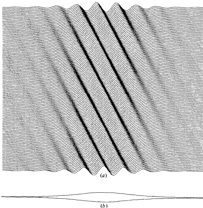
FIGURE 2. (a) One group length of the oblique wave group with parameters \epsilon = 0.05 , k_0 = 10 , \theta = 0.5 , of the first family below the critical angle. Horizontal contraction 10\pi . (b) Envelope of the above group, which is almost identical with the corresponding envelope solution (dn form) of the nonlinear Schrödinger equation.
