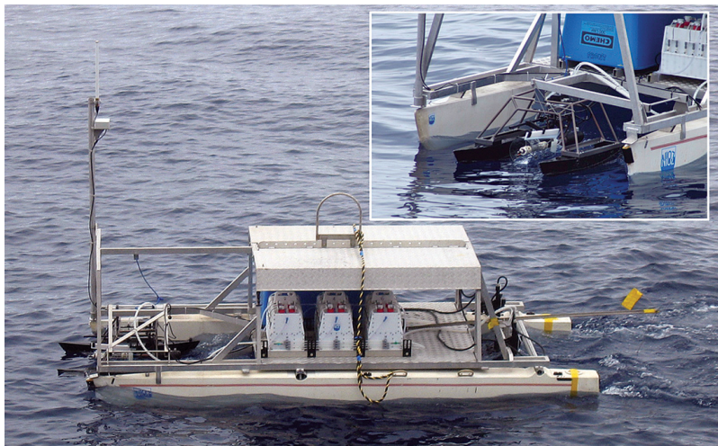
FIG. 5. The remote-controlled catamaran and (inset) close-up of the surface skimmer operating during the second DOGEE cruise.
