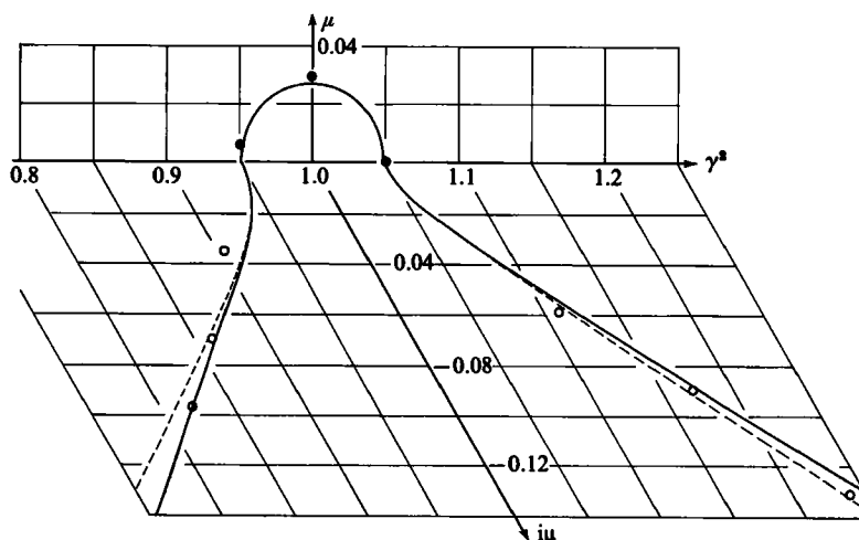
FIGURE 6. Comparison between empirically determined values of \mu and the theoretical predictions (19) (—) and (21) (---). The points ● were determined from decay rates, and ○ from the wavelengths of the envelopes of \tilde{\zeta}(z) shown in figure 4.
