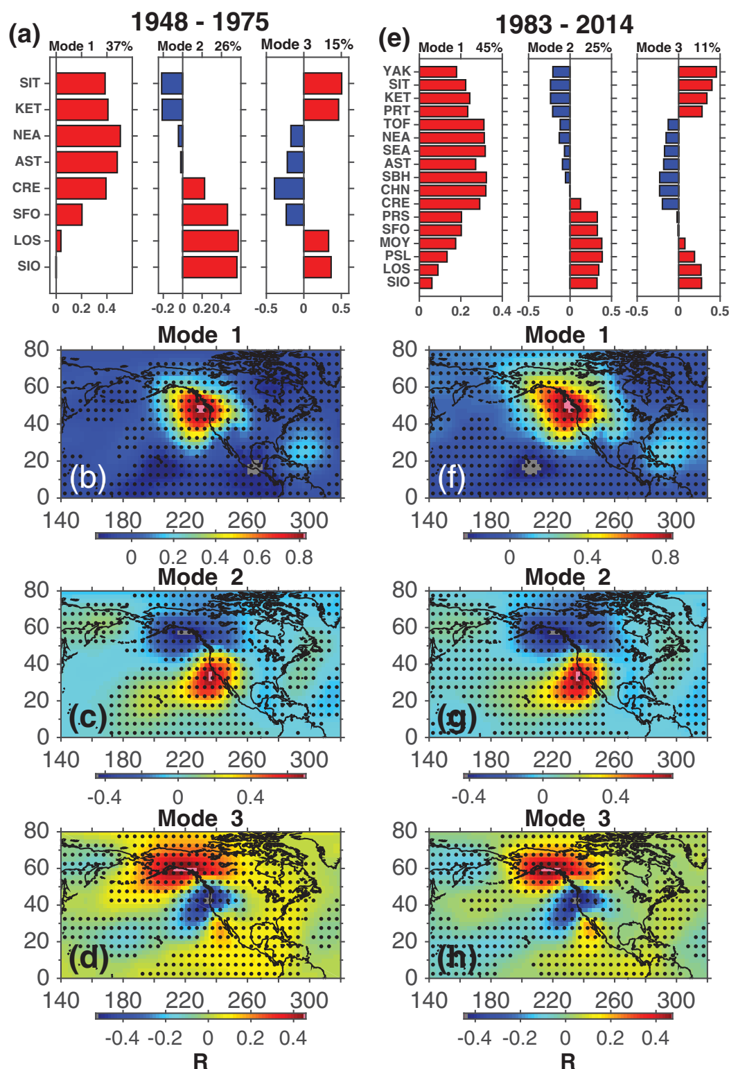
Figure 4. (a) Empirical orthogonal functions (EOFs) of hourly nontide (storm surge) variability over long-duration records during winter (December–February) over the 1948–1975 and 1983–2014 epochs for modes 1–3 from an eight-station tide gauge network along the Pacific coast of North America from La Jolla, CA (SIO) to Sitka, AK (SIT) (see Figure 1 and Table 1 for locations). The percent of variance explained for each mode is given in the subplot title. (b–d) Correlation coefficients ( R ) between respective principal component time series for modes 1–3 in Figure 4a with 6-hourly sea level pressure (SLP) anomalies during respective winter months (December–February). Positive (negative) R is associated with negative (positive) SLP anomalies. Regions where p -values are less than 0.05 are indicated by black dots. (e–h) Same as Figures 4a–4d except for the 1983–2014 epoch. R plots were auto-scaled to emphasize the similarity of correlation patterns between the two epochs.
