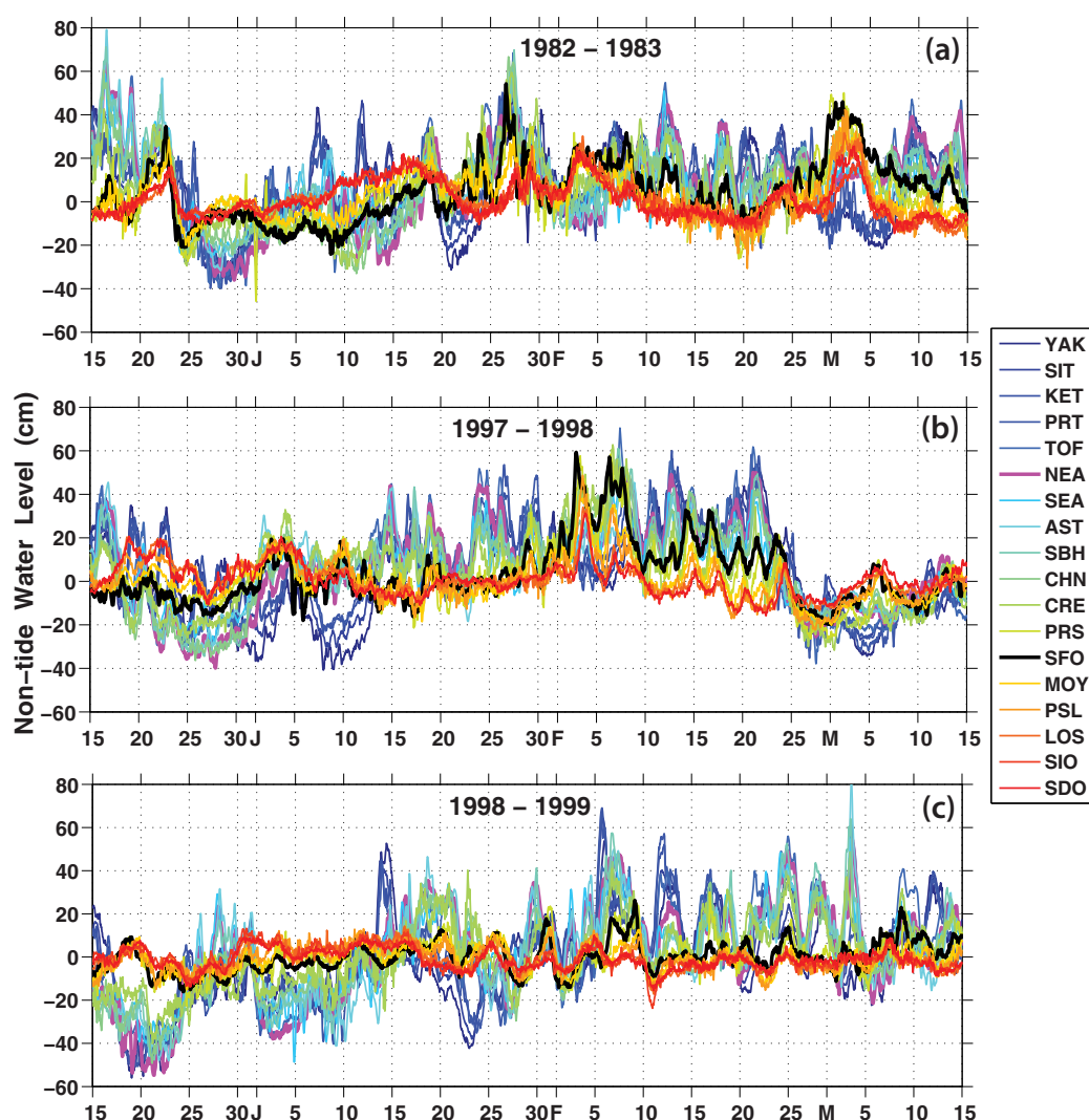
Figure 3. Nontide (storm surge) levels along the Pacific coast of North America during the 1982–1983 and 1997–1998 great El Niños, with the 1998–1999 strong La Niña included for comparison. Coastal stations are color-coded north-to-south (blue to red), with the Neah Bay (NEA, thick magenta) and San Francisco (SFO, thick black) stations identified to help differentiate the dominant regional locations of coastal storm surge activity (see Figure 1 and Table 1 for locations).
