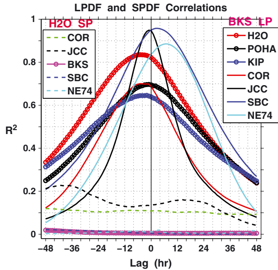
Figure 11. Relationship between coastal and mid-ocean microseism variability over January–June 2002. Lag-correlation curves of RMS vertical displacement spectral levels of long-period double-frequency (LPDF) microseism variability in the [0.11, 0.14] Hz band between coastal station BKS and other coastal and island stations. Also shown are lag correlations of RMS short-period double-frequency (SPDF) variability in the [0.2, 0.3] Hz band between mid-ocean station H2O with coastal stations (see Figures 3 and 4 for locations). COR is located in Corvallis, OR, about 100 km from the coast.
