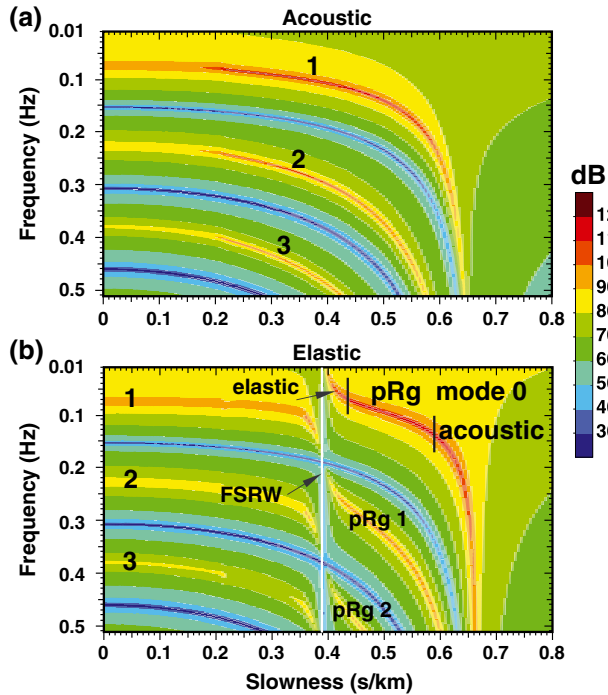
Figure 12. The magnitude of the wave fields in frequency-slowness space for a fluid layer (5 km thick with a sound speed of 1.520 km/s and a density of 1 kg/m 3 ) over (a) a fluid half-space (acoustic (zero shear modulus), with sound speed of 4.730 km/s and density of 3 kg/m 3 ), and (b) a solid half-space (elastic, compressional, and shear speeds of 4.730 and 2.800 km/s, respectively, FSRW wave speed of 2.565 km/s, and a density of 3 kg/m 3 ). The FSRW slowness (0.39 s/km, white line) is the lower slowness bound for pseudo-Rayleigh wave (pRg) modes. Approximate boundaries where fundamental pRg mode 0 exhibits predominantly elastic or acoustic behavior are indicated by vertical black lines, with a transition region between. Acoustic modes 1, 2, and 3 are common to Figures 12a and 12b. Although the fluid half-space in Figure 12a is unrealistic, comparison of these cases shows the effect of shear. Source and receivers are 0.050 km above the interface. These plots were computed using a seismo-acoustic fast-field algorithm [Schmidt, 1988].
