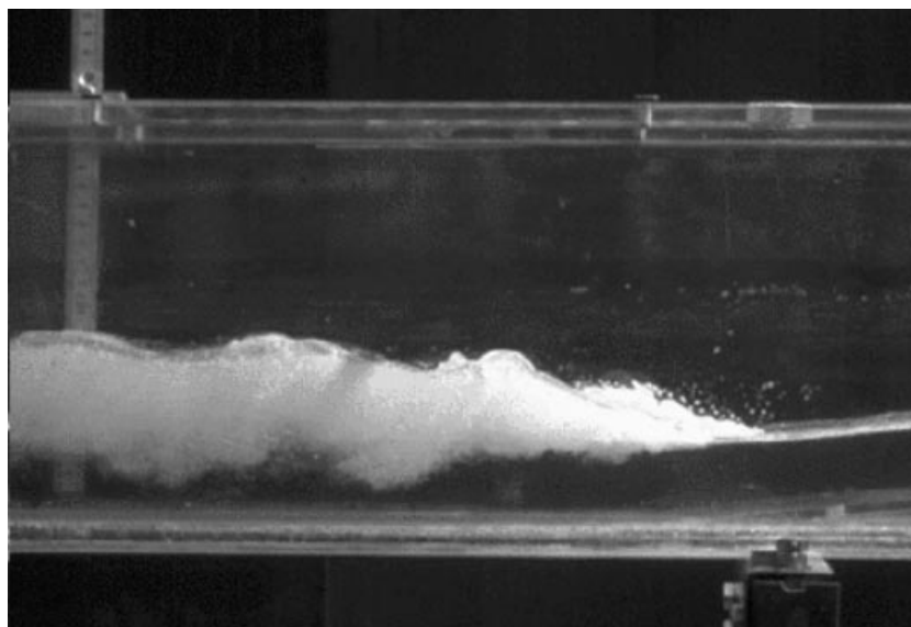
FIGURE 6. Photograph of a hydraulic jump. This is the same flow as shown in Part 1 figure 5, but in this case there was a layer of tiny bubbles on top of the water entering the breaker. The bubbles were sufficiently small that they took more than five minutes to rise 10 cm in water at rest, thus they illustrate the extent of the turbulence-induced mixing of the surface water. The vertical scale on the left is marked in cm. The incoming flow is about 4 cm deep.
