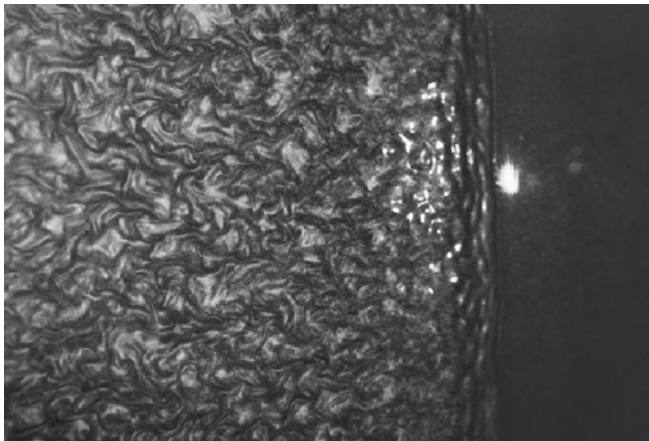
FIGURE 6. Small bore of a few millimetres height in water of comparable depth with flow visualization using aluminium flakes. The field of view is approximately 30 cm long.
