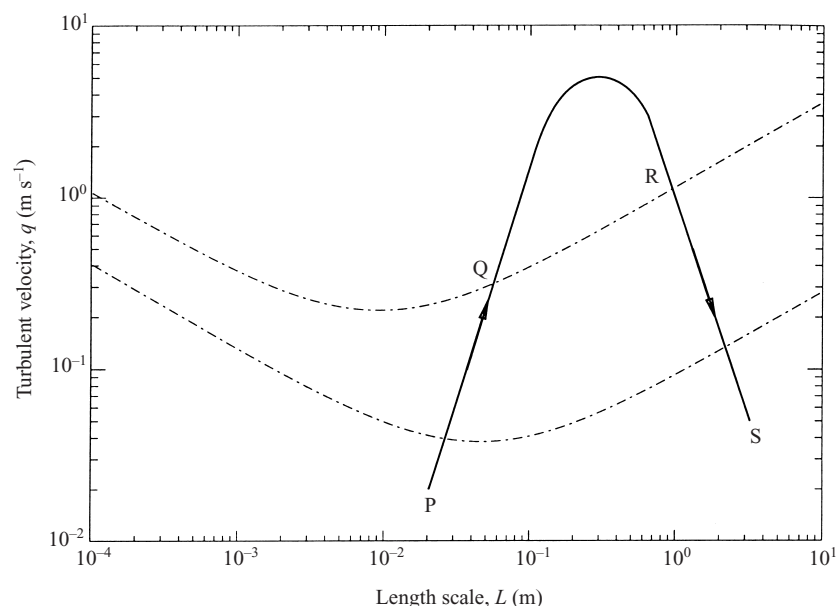
FIGURE 15. Diagram of the (L, q) -plane with a trajectory representative of the surface disturbance due to the flow of a submerged jet. PQRS are points along the surface trace of the centreline of the jet.
