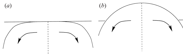
FIGURE 9. Examples of inviscid flows with vortex sheets leaving the free surface. In this idealized limit the flow at the outer edges of the free surface in each diagram is at rest.
