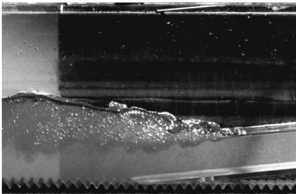
FIGURE 2. Photograph of a hydraulic jump on a flow entering from the right. The volume of turbulence originating at the free surface is marked by dye.
