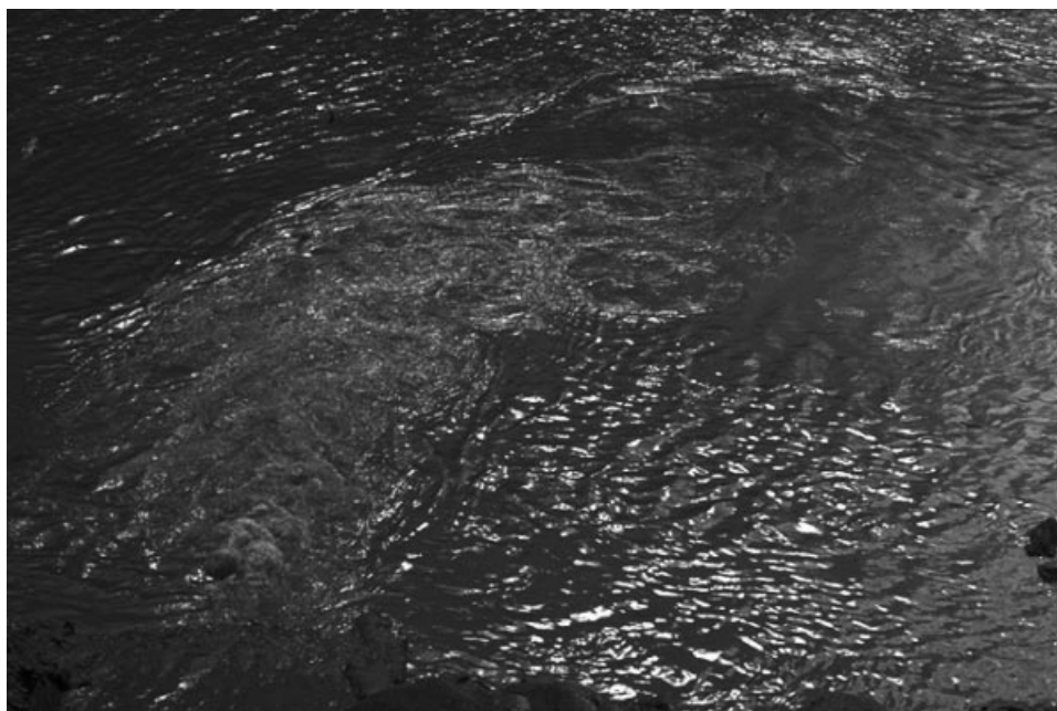
FIGURE 14. The surface traces of a submerged jet entering the River Avon at Bristol. This view covers about 10 m from the river bank which is at the lower edge of the photograph.
