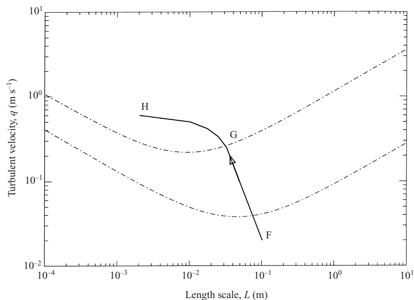
FIGURE 13. Diagram of the (L, q) -plane with a trajectory representative of the flow in a spillway. The points F, G and H represent the initial flow and points further down the spillway respectively.
