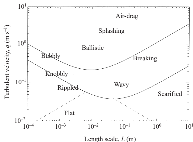
FIGURE 10. Diagram of the (L, q) -plane with tentative descriptions of the flow regimes. The transition region from the upper and lower bounds obtained from equations (3.1) and (3.2) is indicated.
