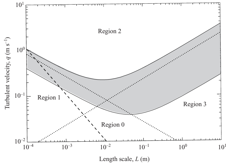
FIGURE 4. Diagram of the (L, q) -plane for water. The shaded area represents the region of marginal breaking and has been obtained by using the two estimated values for both the critical Weber number [(\pi - 2)/5 < We_c < \pi/4] and the critical Froude number [(5/2 - \pi/2)/250 < Fr_c < \pi/24] obtained from equations (3.1) and (3.2). The two straight dotted lines represent a simplified division of the plane for purposes of discussion. The dashed line represents Re = 100 .
