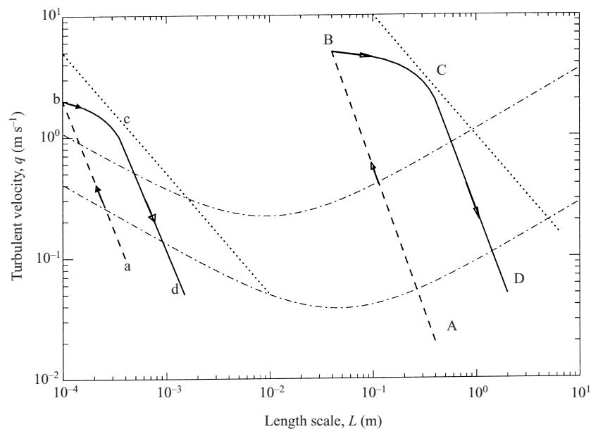
FIGURE 12. Diagram of the (L, q) -plane with trajectories representative of the flow in a hydraulic jump or spilling breaker. The dotted line corresponds to an upper limit to the turbulent energy for each of the two jumps trajectories, ABCD and abcd shown.
