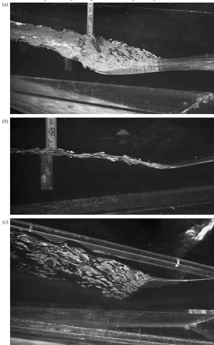
FIGURE 5. Knobbly flow. Oblique view from above (a), side view (b) and view from below (c) of a hydraulic jump fed by flow over a weir. The incoming flow has a depth of about 4 cm. The vertical ruler, visible in the upper two photographs, is marked in centimetres. These photographs are from experiments at the Technical University of Denmark upon which the discussions of Peregrine & Svendsen (1978) were based.
