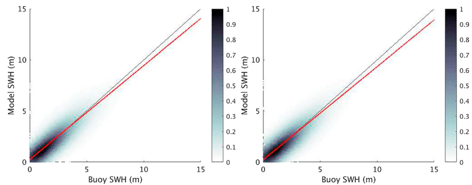
Figure 3. Density scatter plots of SWH (m) from the global model (left) and regional model (right), comparison of modeled (y axis) and observed data (x axis). The 1:1 line is plotted in black and a linear fit to data in red. SWH = significant wave height.
