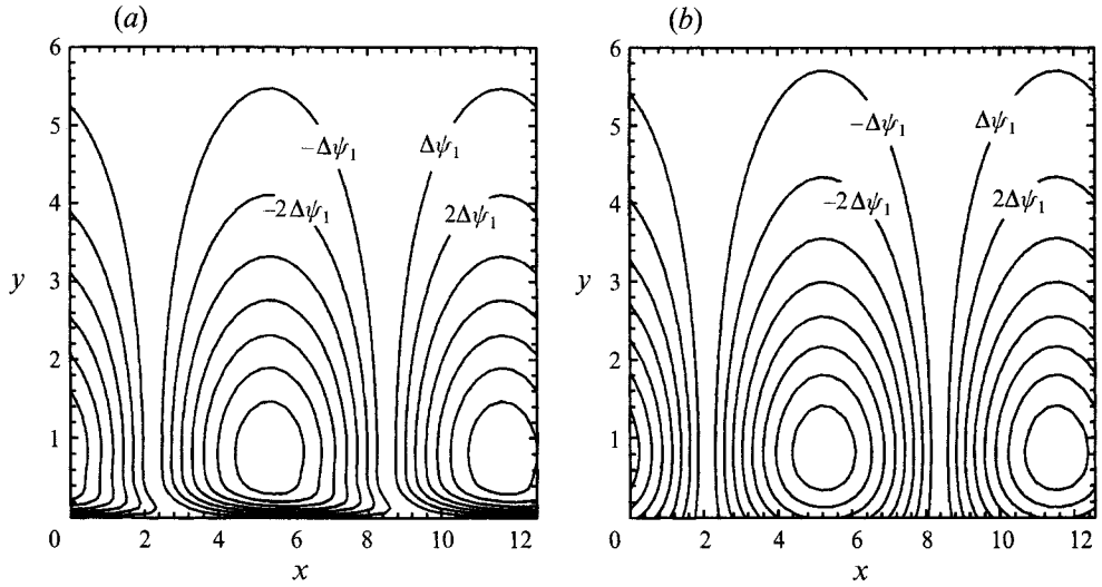
FIGURE 12. Spatial structure of the correction to the stream function induced by a wall waviness in Stokes flow (\psi_1(x, y, t)) : R_g = 500 , \alpha = 0.5 , t = 0 . Outer region, O(y) = 1 . (a) Equation (18), (b) equation (A 3) ( \Delta\psi_1 = 0.04 ).
