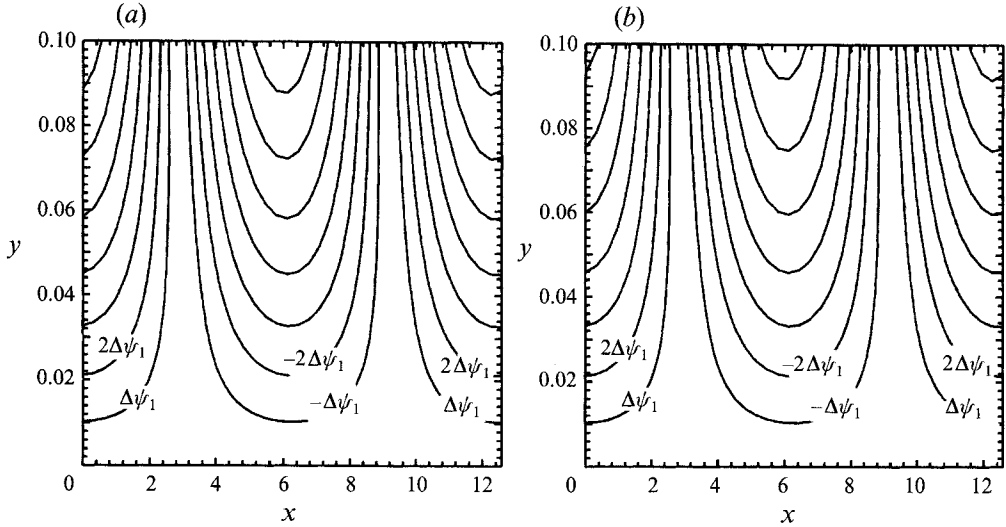
FIGURE 13. As figure 12 but for the inner region, O(y) = R_\delta^{-1/3} . (a) Equation (18), (b) equation (A 9) ( \Delta\psi_1 = 0.02 ).
