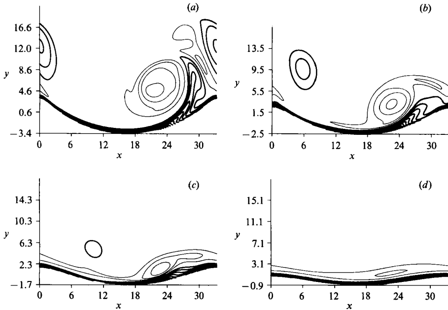
FIGURE 10. Vorticity contours at t = 2\pi : \Delta\omega = 0.15 (—, clockwise vorticity; ---, counter-clockwise vorticity) R_\delta = 50 , s^*/l^* = 0.75 . (a) h^*/l^* = 0.20 ; (b) h^*/l^* = 0.15 ; (c) h^*/l^* = 0.10 ; (d) h^*/l^* = 0.05 .
