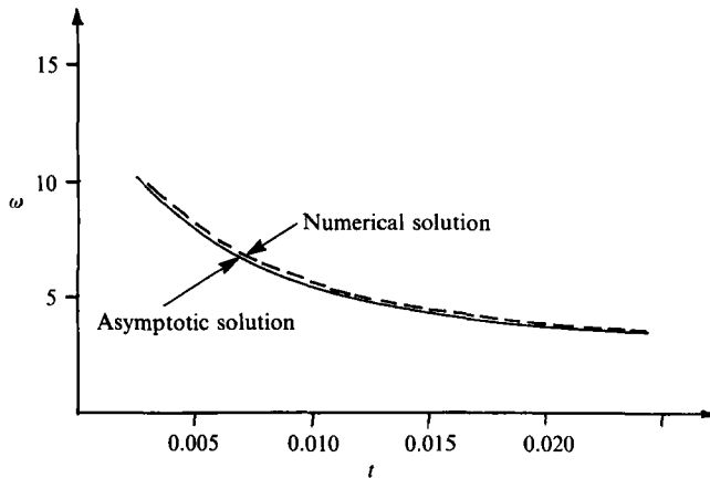
FIGURE 3. Vorticity time development at the ripple trough ( R_\delta = 50 , h = 5.0 , l = 33.33 ).
