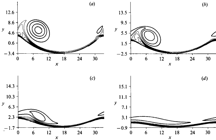
FIGURE 9. Vorticity contours at t = \pi : \Delta\omega = 0.15 (—, clockwise vorticity; ---, counter-clockwise vorticity) R_\delta = 50 , s^*/l^* = 0.75 . (a) h^*/l^* = 0.20 ; (b) h^*/l^* = 0.15 ; (c) h^*/l^* = 0.10 ; (d) h^*/l^* = 0.05 .
