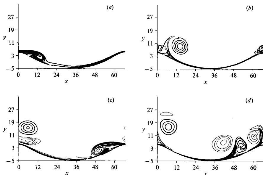
FIGURE 7. Vorticity contours: \Delta\omega = 0.15 (—, clockwise vorticity; ---, counterclockwise vorticity), R_b = 100 , h^*/l^* = 0.15 , s^*/l^* = 0.75 . (a) t = \frac{1}{2}\pi ; (b) t = \pi ; (c) t = \frac{3}{2}\pi ; (d) t = 2\pi .
