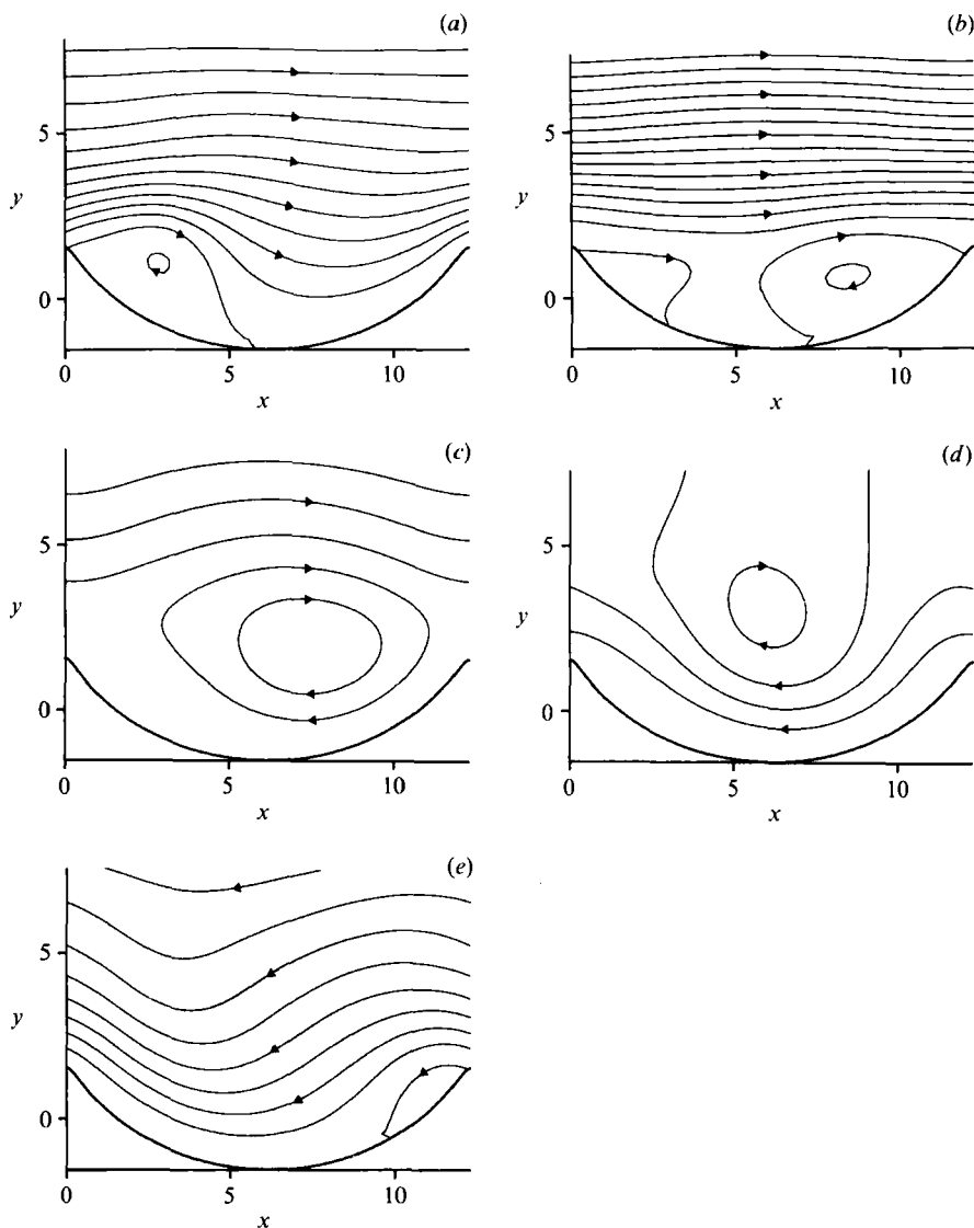
FIGURE 14. Streamline time development ( R_\delta = 48.75 , h = 3.07 , l = 12.27 ). (a) t = 0.628 ; (b) t = 1.571 ; (c) t = 2.827 ; (d) t = 3.142 ; (e) t = 3.456 .
