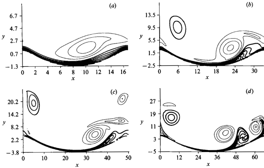
FIGURE 13. Vorticity contours at t = 2\pi : \Delta\omega = 0.15 (—, clockwise vorticity; —, counter-clockwise vorticity) h^*/l^* = 0.15 , s^*/l^* = 0.75 . (a) R_\delta = 25 ; (b) R_\delta = 50 ; (c) R_\delta = 75 ; (d) R_\delta = 100 .
