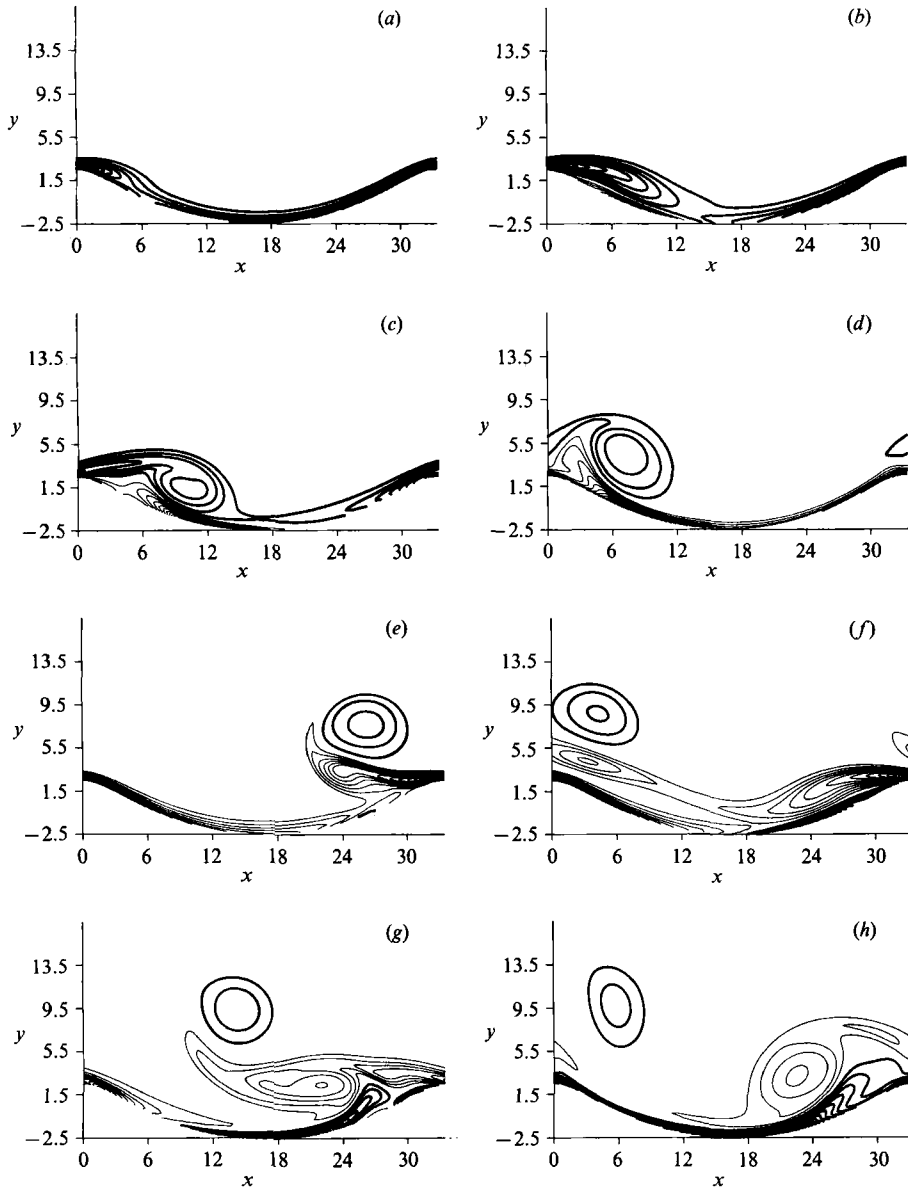
FIGURE 6. Vorticity contours: \Delta\omega = 0.15 (—, clockwise vorticity; ---, counterclockwise vorticity), R_\delta = 50 , h^*/l^* = 0.15 , s^*/l^* = 0.75 . (a) t = \frac{1}{4}\pi ; (b) t = \frac{1}{2}\pi ; (c) t = \frac{3}{4}\pi ; (d) t = \pi ; (e) t = \frac{5}{4}\pi ; (f) t = \frac{3}{2}\pi ; (g) t = \frac{7}{4}\pi ; (h) t = 2\pi .
