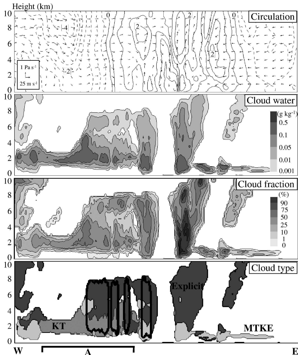
FIG. 7. Vertical cross sections along line W-E in Fig. 3 from the 72-h CTRL forecast valid at 0000 UTC 9 Feb 2003. (top) The along- and across-line circulations, with arrows and contours (every 0.5 \text{ m s}^{-1} ) respectively. (second from top) The total cloud water ( \text{g kg}^{-1} ), (third from top) the total cloud fraction (%), and (bottom) the dominant cloud type. The along-line circulations are relative to the main precipitation band motion (i.e., a mean propagation speed of 8 \text{ m s}^{-1} was subtracted from the east-west wind component). The cloud type was determined as in Fig. 6. All the above meteorological quantities were averaged in the cross-line direction, and these panels thus in fact represent mean vertical cross sections along a 500-km band following line W-E.
