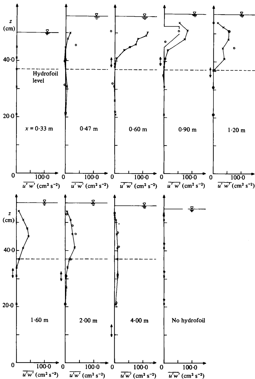
FIGURE 4. Vertical profiles of \overline{u'w'} in sections at various distances downstream of the hydrofoil. The profile in the lower right-hand corner is for the flow in absence of a hydrofoil. x, full-scale experiment; O, half-scale experiment.
