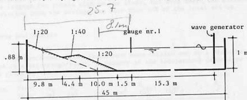
Fig. 2 - Sketch of wave flume with bar-trough beach profile (plane slope indicated by dashed line)
