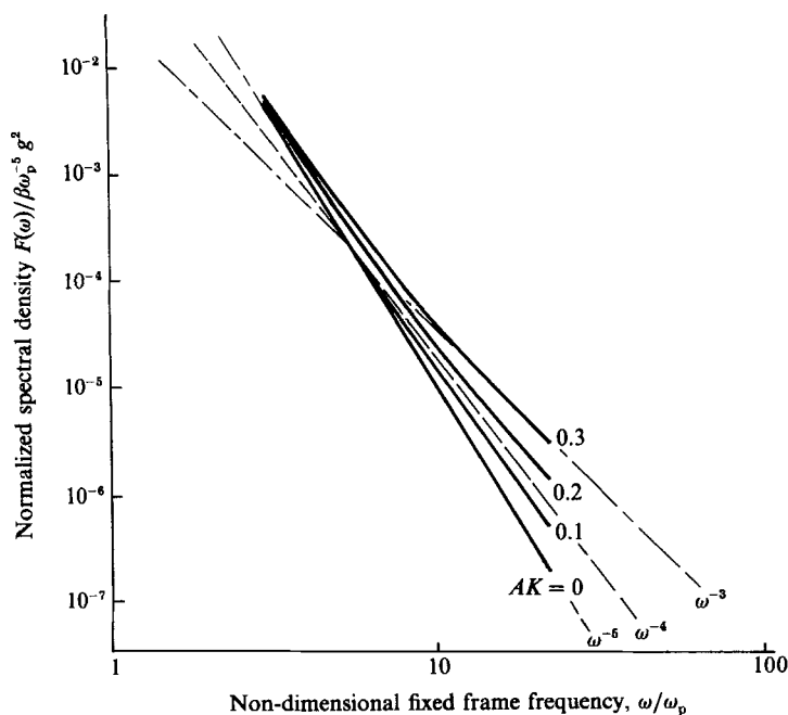
FIGURE 8. Computed normalized frequency spectra as a function of the dominant waveslope AK for a two-dimensional short-wavenumber spectrum of the form given by equation (7.2). The effects shown are entirely the result of kinematic Doppler distortion. \beta is the Phillips constant.
