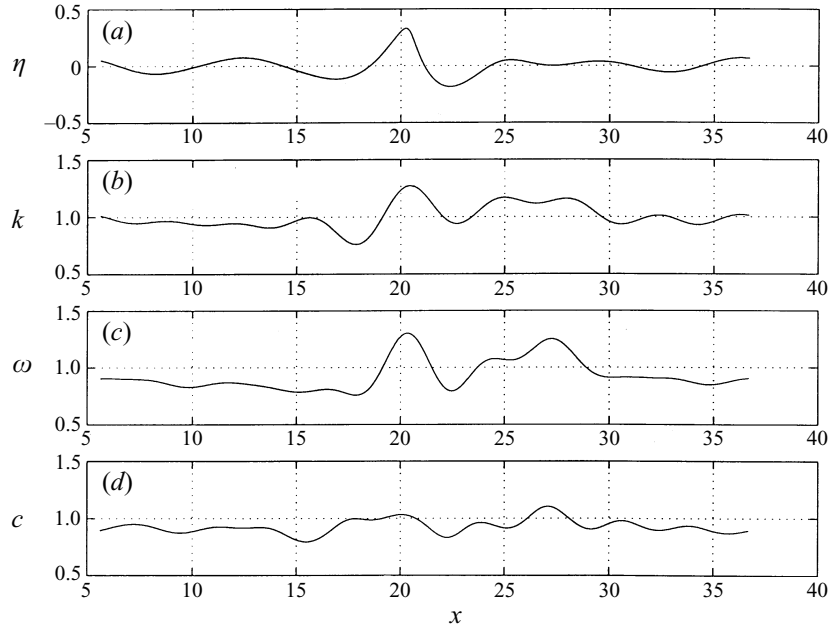
FIGURE 7. Horizontal distribution of propagation characteristics just prior to the commencement of recurrence at t/2\pi = 84.4 for the case shown in figure 1: (a) wave elevation profile, (b) local wavenumber k , (c) local frequency \omega , (d) local phase speed c .
