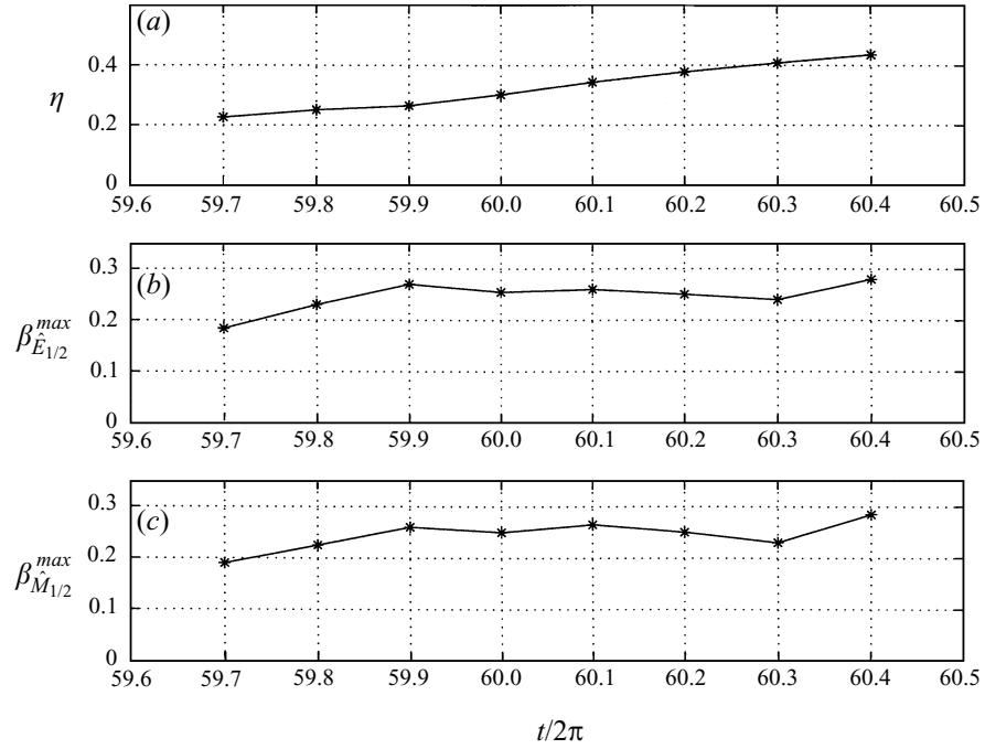
FIGURE 15. As figure 14 but for the temporal evolution of \beta^{max} during the time interval t/2\pi \in (59.7, 60.4) with breaking occurring at the next time step ( t/2\pi = 60.5 ).
