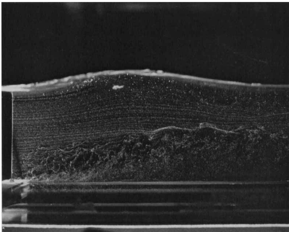
FIGURE 6. Streak lines in a small scale breaking wave. For identification, see figure 7.
