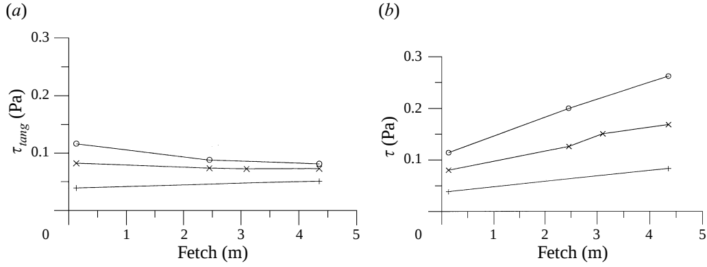
FIGURE 9. (a) Tangential stress versus fetch. Wind speeds: +, 4.8 m s -1 ; ×, 6.3 m s -1 ; ○, 8.1 m s -1 . (b) Total stress versus fetch. Wind speeds: +, 4.8 m s -1 ; ×, 6.3 m s -1 ; ○, 8.1 m s -1 .
