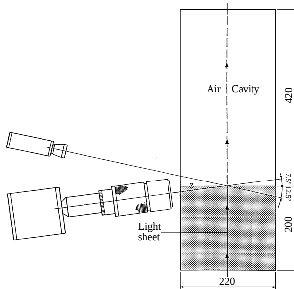
FIGURE 3. Section through wave tank showing alignment of light sheet and cameras. The PIV camera is on the lower left-hand side, looking upward. The smaller videocamera on the upper left-hand side captures the wave profile.
