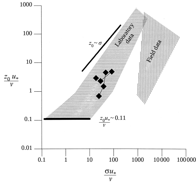
FIGURE 13. The results of this study superimposed on figure 11 of Donelan (1990), showing the roughness Reynolds number z_0 u_* / \nu plotted against the normalized r.m.s. wave height \sigma u_* / \nu . ♦, present results. The scatter of laboratory and open ocean data from previous studies is indicated by the labelled hatched areas. Note that the present wave-free very short fetch data is not shown and lies well to the left of the ordinate axis close to the indicated smooth-wall asymptote.
