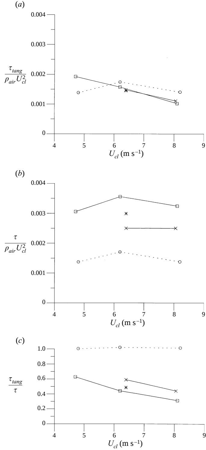
FIGURE 11. (a) Tangential drag coefficient against U_{cl} . Fetches: ○, 0.13 m; ×, 2.45 m; *, 3.10 m; □, 4.35 m. (b) Total drag coefficient against U_{cl} . Fetches: ○, 0.13 m; ×, 2.45 m; *, 3.10 m; □, 4.35 m. (c) Stress ratio \tau_{tang}/\tau against U_{cl} . Fetches: ○, 0.13 m; ×, 2.45 m; *, 3.10 m; □, 4.35 m.
