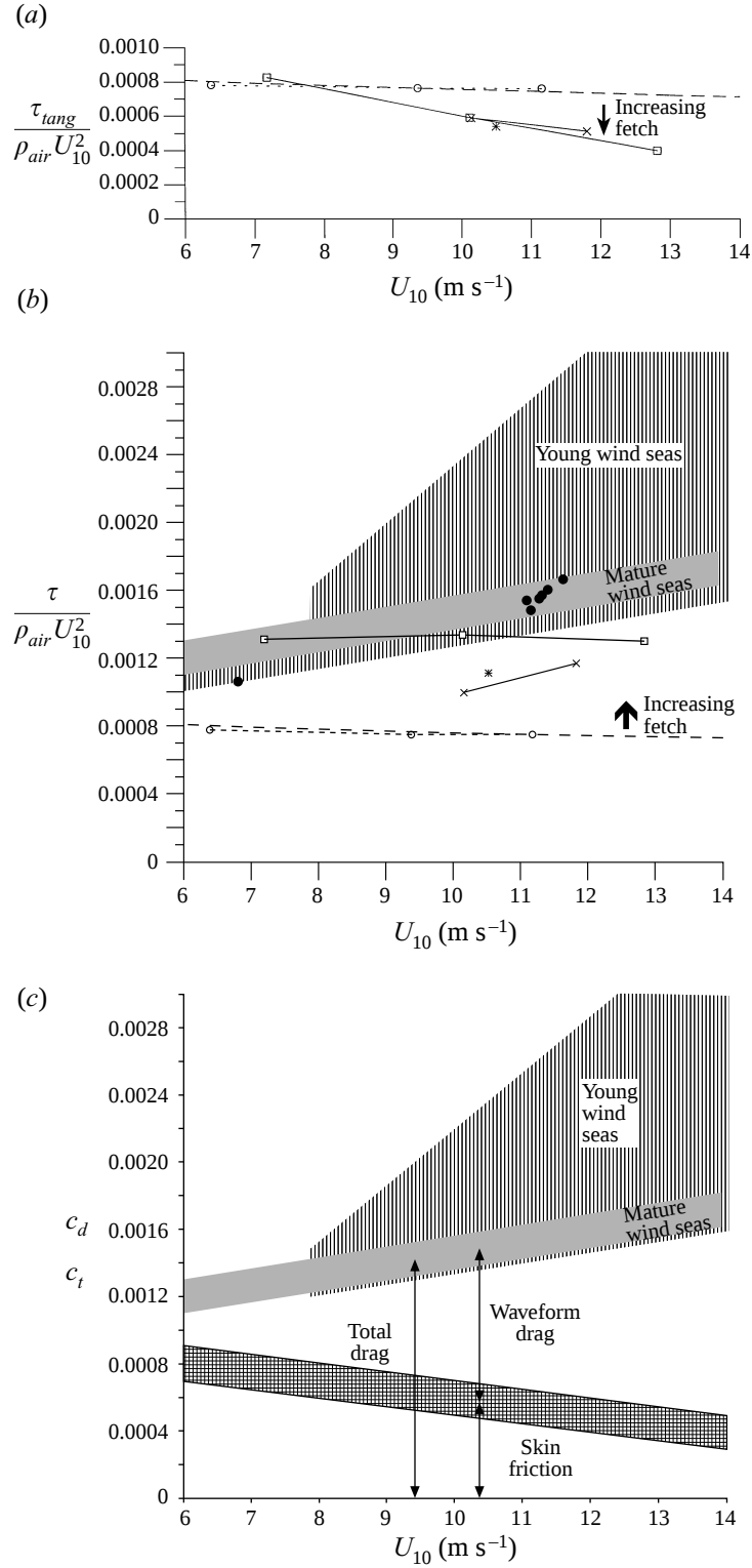
FIGURE 12. (a) Tangential drag coefficient versus U_{10} . Fetches: ○, 0.13 m; ×, 2.45 m; *, 3.10 m; □, 4.35 m. The corresponding curve for turbulent flow over smooth walls is indicated by the dashed
