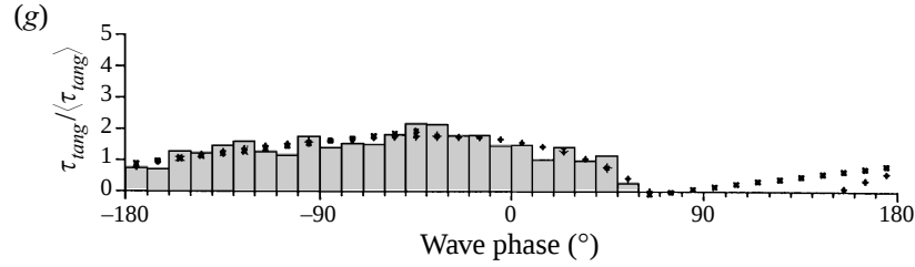
FIGURE 5. Average waveforms with distributions as a function of wave phase of: surface velocity; tangential stress; 10^\circ binned tangential stress; and, 10^\circ binned wave coherent tangential stress. The smoothed ‘inner’ and ‘outer’ interpolated distributions of tangential stress used to derive the revised mean tangential stresses in table 1 are shown as +, \times , respectively, in the fourth panel in each case. The basis for these smoothed interpolations is shown in figure 5(g). (a) Wind speed 4.8 \text{ m s}^{-1} , fetch 4.35 \text{ m} . (b) Wind speed 6.3 \text{ m s}^{-1} , fetch 2.45 \text{ m} . (c) Wind speed 6.3 \text{ m s}^{-1} , fetch 3.10 \text{ m} . (d) Wind speed 6.3 \text{ m s}^{-1} , fetch 4.35 \text{ m} . (e) Wind speed 8.1 \text{ m s}^{-1} , fetch 2.45 \text{ m} . (f) Wind speed 8.1 \text{ m s}^{-1} , fetch 4.35 \text{ m} . (g) Smoothed interpolations of the normalized tangential stress shown in relation to the normalized tangential stress distribution for the ensemble of all data sets. +, \times represent the ‘inner’ and ‘outer’ fits described in the text.
