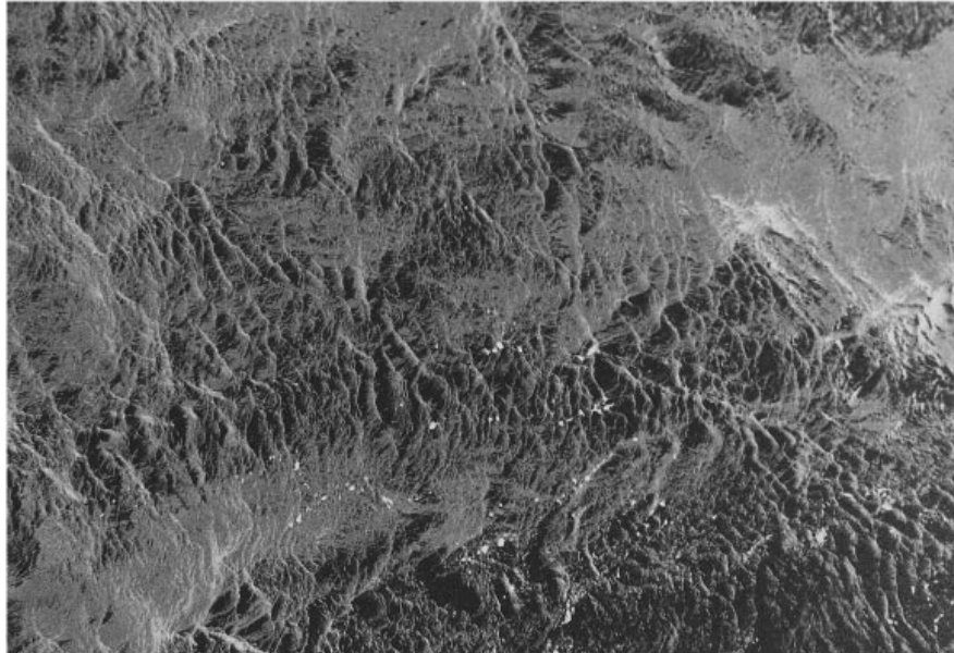
FIGURE 1. A close range photograph from 6 m above the sea surface showing its fine structure for open ocean wave conditions of 3 m significant wave height with a wind speed of 12 \text{ m s}^{-1} from the top right to the lower left. The field of view is 4 \text{ m} \times 2.6 \text{ m} , indicating microscale breakers with 50 mm to 150 mm wavelengths.
