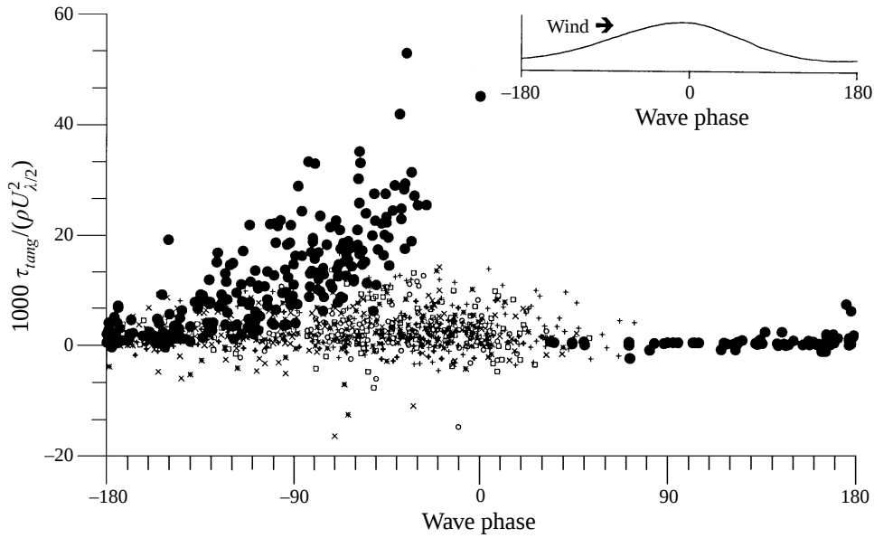
FIGURE 7. Estimates of surface tangential stress normalized by the wind speed half a wavelength above the mean water level from ●, Okuda et al. 1977 and this study: +, wind speed 4.8 m s -1 , fetch 4.35 m; ×, wind speed 6.3 m s -1 , fetch 2.45 m; *, wind speed 6.3 m s -1 , fetch 3.10 m; □, wind speed 6.3 m s -1 , fetch 4.35 m; ○, wind speed 8.1 m s -1 , fetch 2.45 m; +, wind speed 8.1 m s -1 , fetch 4.35 m.
