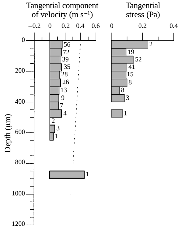
FIGURE 6. Distributions of velocity and tangential stress binned by distance from the interface. Fetch 4.35 m, wind speed 6.3 \text{ m s}^{-1} . The slope of the dashed line indicates the expected rate of change of velocity away from the interface based on the mean measured tangential stress. The numbers to the right-hand side of each bar indicate the number of samples in each bin.
