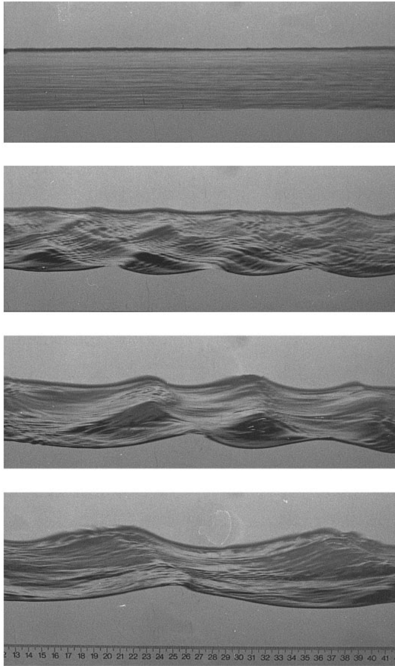
FIGURE 2. Photographs of wave conditions within the laboratory flume. The wind and waves are moving from left to right. From the upper to lower panel: wind speed 8.1 \text{ m s}^{-1} , fetch 0.13 \text{ m} ; wind speed 4.8 \text{ m s}^{-1} , fetch 4.35 \text{ m} ; wind speed 6.3 \text{ m s}^{-1} , fetch 4.35 \text{ m} ; wind speed 8.1 \text{ m s}^{-1} , fetch 4.35 \text{ m} .
