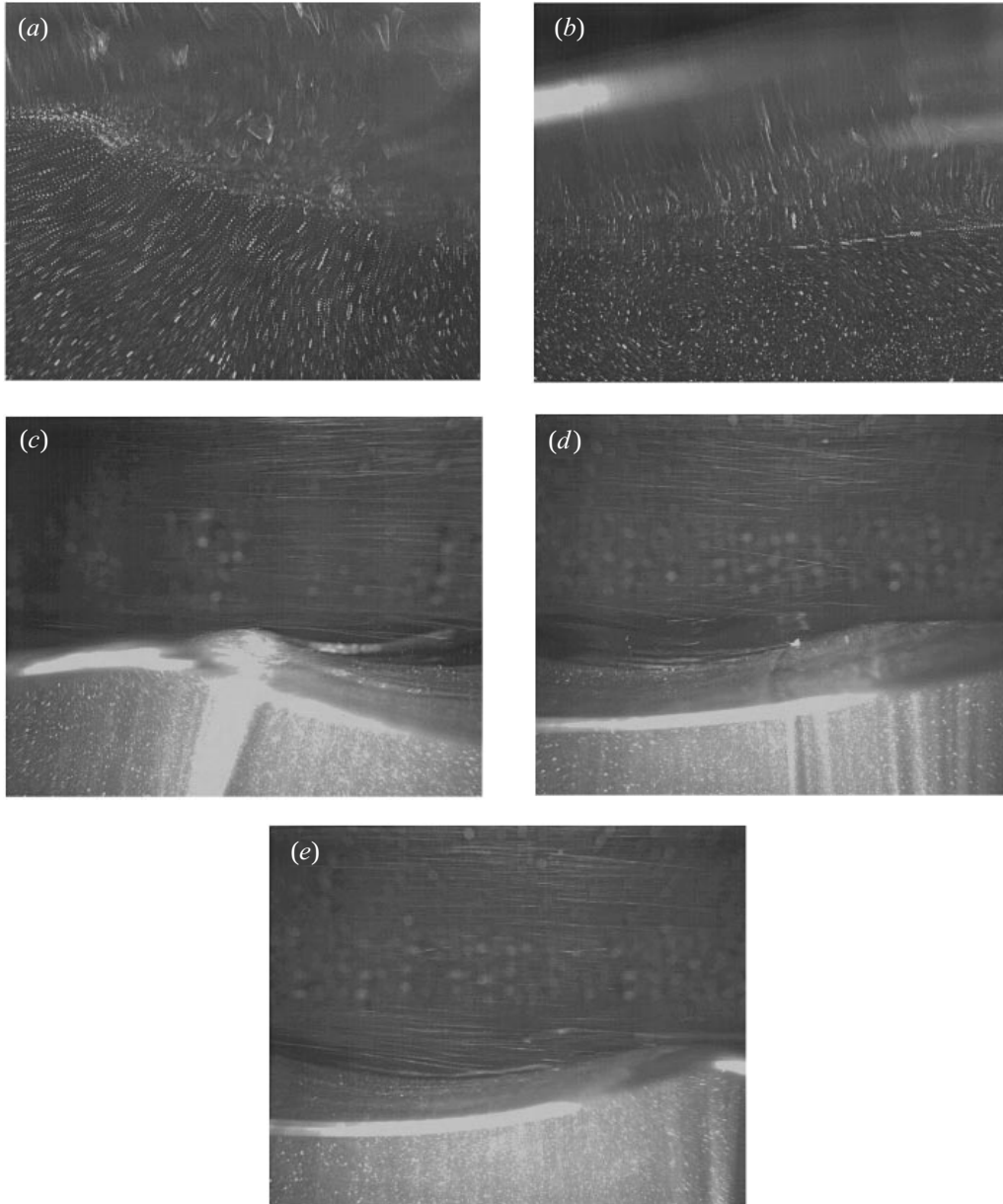
FIGURE 8. (a) and (b) show aqueous PIV images of the trough regions downwind of small-scale breaking wave crests at the 2.45 m fetch. The wind and waves are travelling from left to right, with the breaking crest on the left-hand side of the images. (c)–(e) show visualizations of water particles in the air flow above the wave surface, at the 4.35 m fetch. In the immediate foreground is the meniscus on the tank wall. The bright continuous line above this is the light-sheet interface with some near-surface particles visible. The bright streaks in the upper half of the pictures are water particles injected in the air flow. Droplets have been deposited on the tank wall creating bright spots in that region. (a) PIV image of trough region showing the lack of any organized viscous sublayer surface flow, confirming that this is a region of negligible tangential stress ( U_{cl} = 8.1 \text{ m s}^{-1} ). (b) PIV image of trough region again showing the lack of any organized viscous sublayer surface flow. In addition, the flow re-attachment on the windward face is clearly visible through the organized viscous sublayer flow seen on the right-hand side of the image ( U_{cl} = 6.3 \text{ m s}^{-1} ). (c) Airflow separation over a breaking crest ( U_{cl} = 8.1 \text{ m s}^{-1} ). (d) Airflow reattachment in the vicinity of the downwind crest. The motion of a few water droplets is visible within the separation zone ( U_{cl} = 6.3 \text{ m s}^{-1} ). (e) Airflow reattachment occurring just downwind of the trough ( U_{cl} = 6.3 \text{ m s}^{-1} ).
