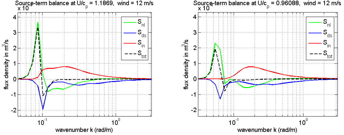
Figure 11. Source term balance for developing seas in period 1 (left panel) and maturing seas period 3 (right panel). Note the even for period 1, the spectral peak dissipation rate due to breaking is considerably larger than the wind input, as discussed in the text.
