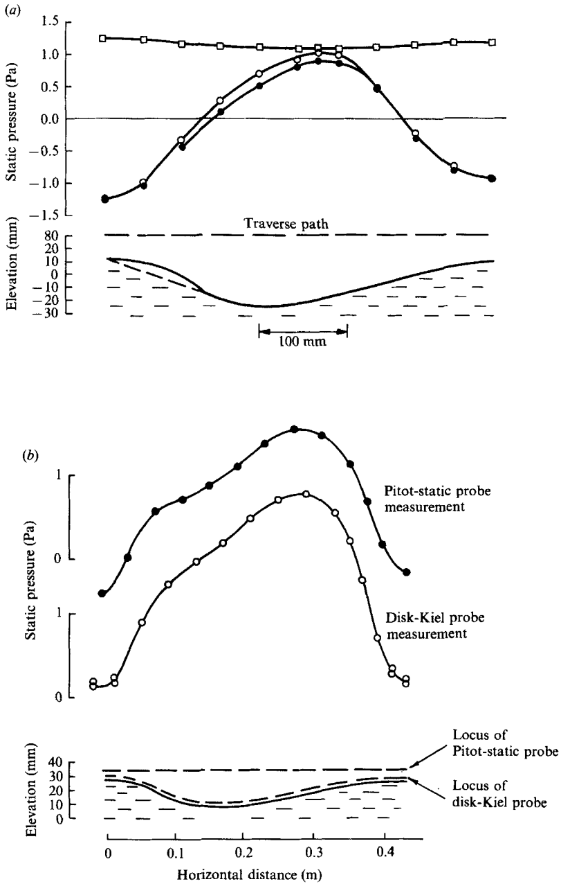
FIGURE 5. Performance comparisons of pressure sensed by \circ , disk-Kiel tube probes and by \bullet , a standard NPL 2.3 mm dia. Pitot-static tube along traverse paths indicated over stationary breaking waves. (a) Pressure and velocity correction term ( \square ) at a fixed height above the mean water level. The centreline windspeed was 5.3 m/s from left to right. (b) Difference between fixed height and surface-following pressure determination. The centreline wind speed was 4 m/s from left to right (after Banner 1986).
