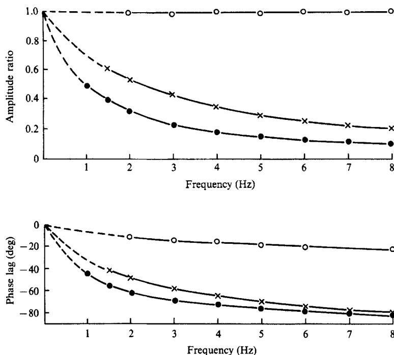
FIGURE 7. Frequency response characteristics for ●, the disk probe, X, Kiel tube probe and O, wave height gauges. Upper curve is the amplitude ratio, lower curve is the phase lag in degrees of the sensed signal with respect to the applied signal.
