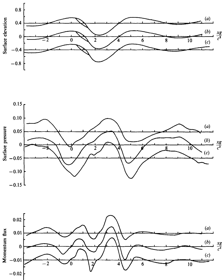
FIGURE 10. Non-dimensional distributions of the mean surface elevation \eta g/c^2 (upper curves), mean surface pressure p/\rho_* U_c^2 (middle curves) and mean local momentum flux p\eta_x/\rho_* U_c^2 (lower curves) for the stationary-wave experiments for different centreline windspeeds (a) U_c/c = 3.29 , (b) U_c/c = 4.81 , (c) U_c/c = 6.84 . The dimensionless horizontal coordinate is xg/c^2 measured downwind from an arbitrary origin at the location of the breaking crest. ( c = 0.79 m/s; g = 9.81 m/s 2 ; \rho_* = 1.225 kg/m 3 ).
