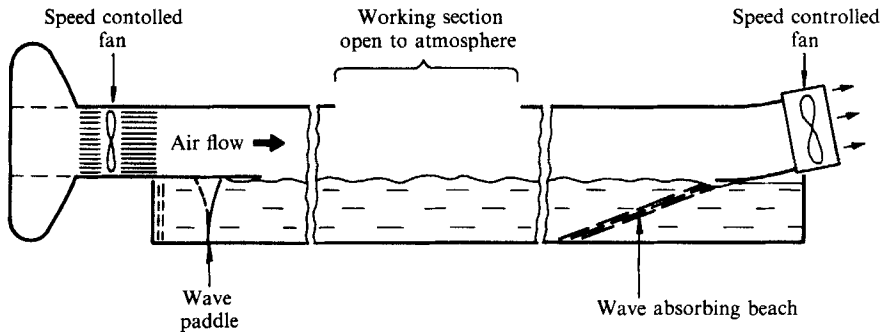
FIGURE 6. Wind-wave flume configuration for propagating wave experiments. Working section open to atmosphere was 0.65 m in length, centred 2.5 m from upwind air flow exit plane. Other dimensions as in figure 1.
