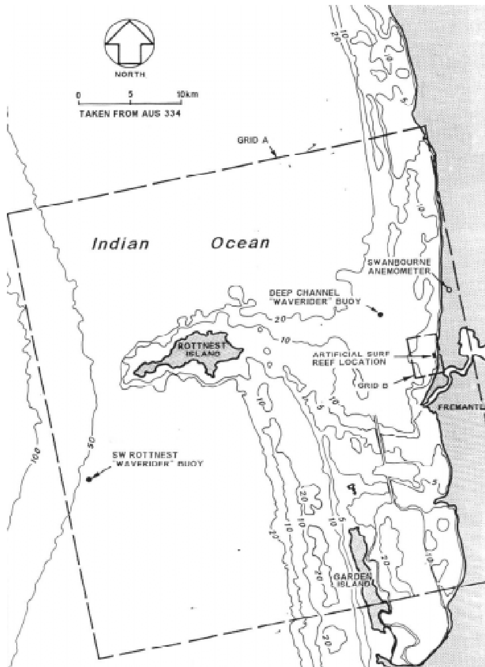
Figure 2.12. Location along the Perth coastline of the Cable Station artificial reef.
