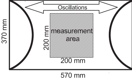
FIG. 1. Sketch of the experiment (Top view). The vessel is translating horizontally with a constant amplitude frequency modulated oscillation, which frequency is chosen in the interval [0.5, 1.5] Hz. Two curved walls are placed on left and right sides to improve the isotropy by diverging waves reflexion
