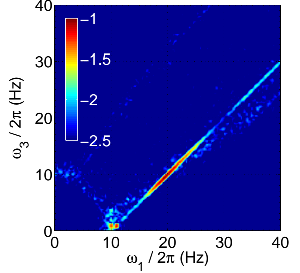
FIG. 4. Representation of 3-wave coherence |C(\omega_1, \omega_2, \omega_3)| (see text for definitions). The specular light blue pattern on the background corresponds to statistical convergence noise so that the statistical convergence is about 10^{-2.5} . Here \omega/2\pi is chosen equal to 10 Hz. Thus the observed line of correlation lies above the convergence level by more than one order of magnitude at the maximum of correlation. This is the sign of the presence of significant 3-wave coupling in the signal. The line lies on the resonance curve \omega_1 = \omega_2 + \omega_3 as expected from such statistical estimator. Color is \log_{10} |C| .
