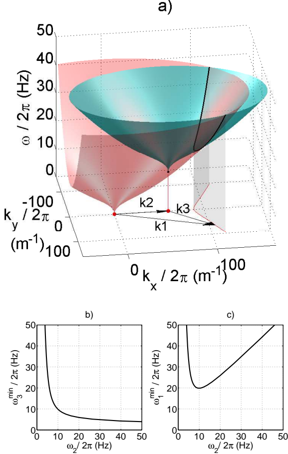
FIG. 3. Solutions for the 3 wave resonances of gravity capillary waves. (a) The red surface corresponds to the dispersion relation (3). First a given value of \mathbf{k}_2 is chosen. The blue surface corresponds then to the sum \omega(\mathbf{k}_2) + \omega(\mathbf{k}_3) . The resonant wave at \mathbf{k}_1 must verify the resonance conditions \mathbf{k}_1 = \mathbf{k}_2 + \mathbf{k}_3 and \omega_1 = \omega_2 + \omega_3 and thus lie on the intersection of the red and blue surfaces (thick black line). The red line at the bottom of the axes corresponds to the projection of the black line. (b) Evolution of \omega_3^{\min}(\omega_2) that is the minimum value of \omega_3 for which there is a possible solution for a given value of \omega_2 . (c) corresponding value \omega_1^{\min} .
