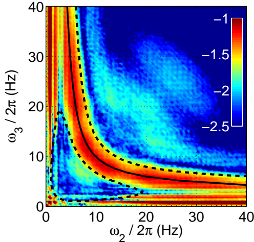
FIG. 5. Bicoherence B(\omega_2, \omega_3) = C(\omega_2 + \omega_3, \omega_2, \omega_3) . The solid black line corresponds to the minimum value \omega_3^{\min}(\omega_2) allowing exact resonances (see text). The dashed line corresponds to the transformation of the solid line when allowing for a \delta k/2\pi = 5 \text{ m}^{-1} uncertainty on the resonance condition (see text).
