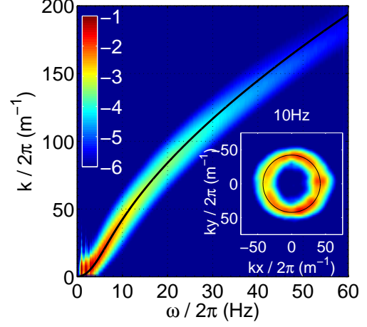
FIG. 2. Space-time Fourier spectrum of the velocity field of the waves E^v(k, \omega) (see text for definition). The color scale is \log_{10} E^v(k, \omega) . The solid black line is the theoretical deep water linear dispersion relation for pure water \omega^2 = gk + \frac{\gamma}{\rho} k^3 with \gamma = 72 \text{ mN/m} . Energy is localized on the dispersion relation and can be observed for frequencies up to 60 Hz. The crossover between gravity and capillary waves occurs at k_c = \sqrt{\rho g / \gamma} = 120\pi corresponding to a wavelength of 1.7 cm and a frequency equal to 13 Hz. Inset: E(\mathbf{k}, \omega) at \omega/2\pi = 10 \text{ Hz} . The energy distribution is fairly isotropic. The black circle corresponds to the linear dispersion relation. Color: \log_{10} E(\mathbf{k}, \omega) between -8 and -4 .
