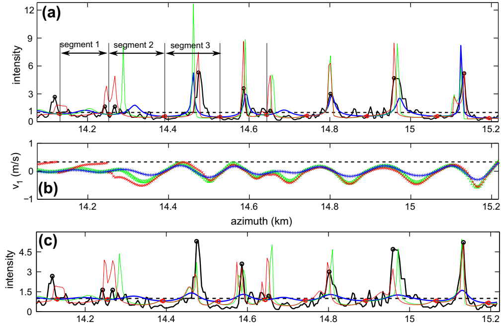
Fig. 5. (a) Example of image intensity as a function of the azimuth for a fixed range (here at i=1 , corresponding to x = 7.488 km), starting from C_1 = 0.7 , and (b) corresponding adjustments of the vertical velocity v_1 . Starting from a linearized inverse SAR transform that gives v_{1,\text{lin}} in blue, the next adjustments include a correction for the low intensity values (in green), a shift of the peaks (in red). (c) is the same as (a) but using a lower linear first guess, with C_1 = 0.3 . The black circles mark the peaks of the image intensity used to define wave segments for the nonlinear adjustment of the velocity v_1 .
