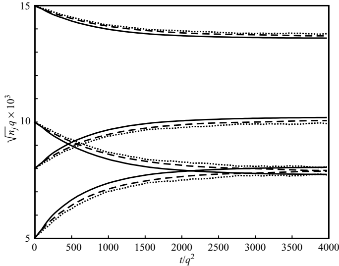
FIGURE 7. Evolution of amplitudes of four wave packets (3.1), normalized by q^{-1} , for q = 1 (solid curves), q = 0.5 (dashed curves), q = 2 (dotted curves), with time scales normalized by q^2 . The averaging is over 50000 realizations.
