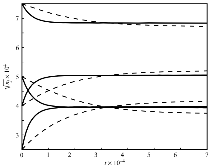
FIGURE 6. As in figure 3(b), but for initial amplitudes of all wave packets multiplied by 0.5.
