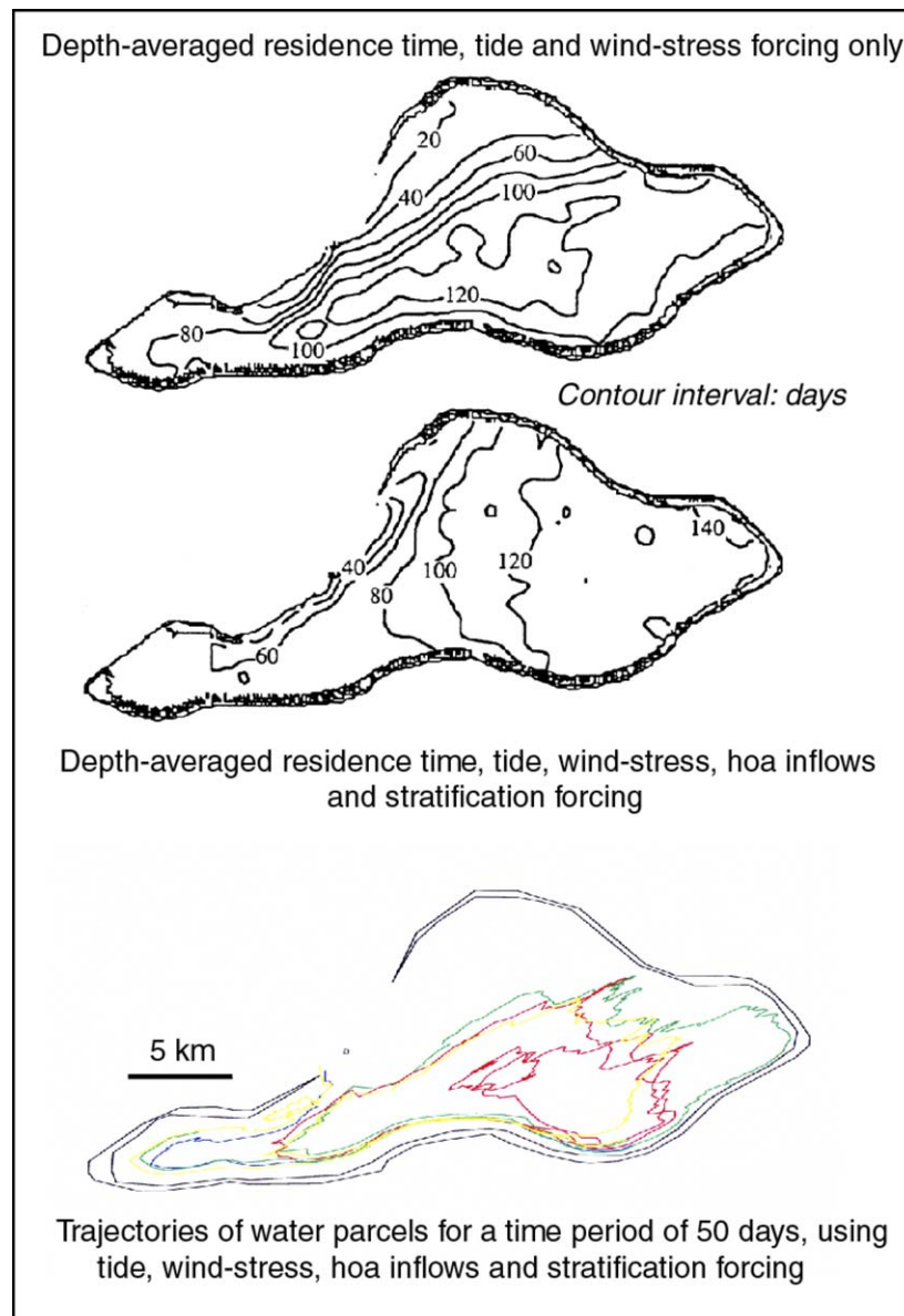
Fig. 8. Examples of 2D products from Moruroa 3D model: atoll residence time and particle tracking sensitivity study to different forcing factors such as wind, tide, hoa inflows and stratification (from Tartinville et al., 1997).
