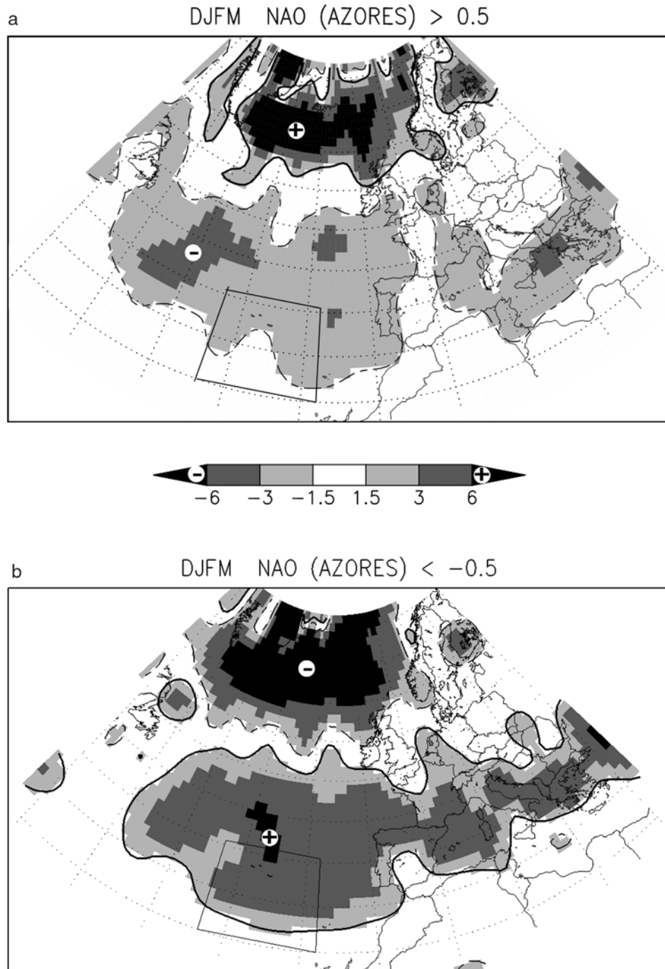
Figure 5 Number of cyclones per winter (DJFM), detected within boxes of 5°longitude × 5°latitude and normalized for 50°N (period 1958–2000). (A) NAO > 0.5; (B) NAO < -0.5. NAO index defined between Ponta Delgada (Azores) and Stykkisholmur (Iceland)
