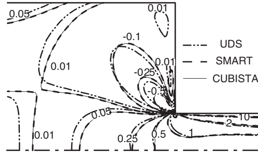
Figure 18. Contours of the first normal stress difference (\tau_{xx} - \tau_{yy})/(3\eta U_2/H_2) obtained with the UDS, SMART and CUBISTA schemes on mesh M1.
