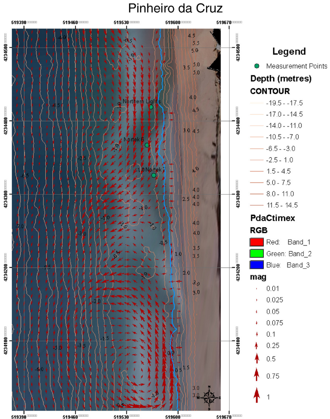
Fig. 13. Time-lapsed imagery with Delft3D output as an overlay. Red arrows depict the magnitude and direction of the current. The coordinate system is in UTM.
