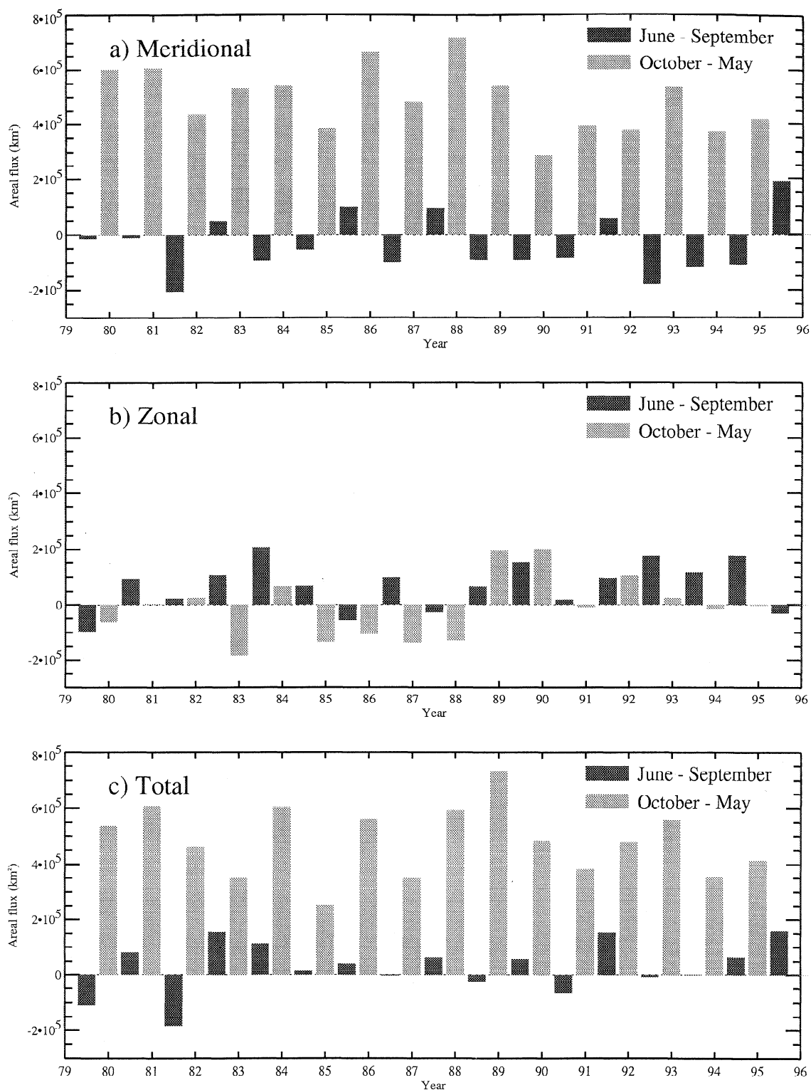
Figure 8. Model-derived (a) meridional, (b) zonal, and (c) total areal ice fluxes for the winter (October to May) and summers seasons (June to September) during the period 1979 to 1995.
