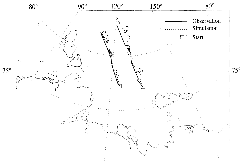
Figure 3. Comparison of satellite-derived and calculated trajectories of giant ice floes in the central part of the Laptev Sea for the period October 28, 1987, to May 6, 1988.
