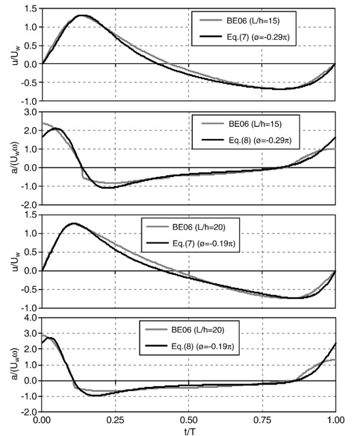
Fig. 11. Comparison of orbital velocity and acceleration time series computed from Eq. (7) and (8), and BE06 with H/h = 0.4 , h = 2 m, slope 1:40, and varying L/h . The reproduction with Eq. (7) and (8) are accomplished with \phi = -0.29\pi and r = 0.699 , and \phi = -0.19\pi and r = 0.784 .
