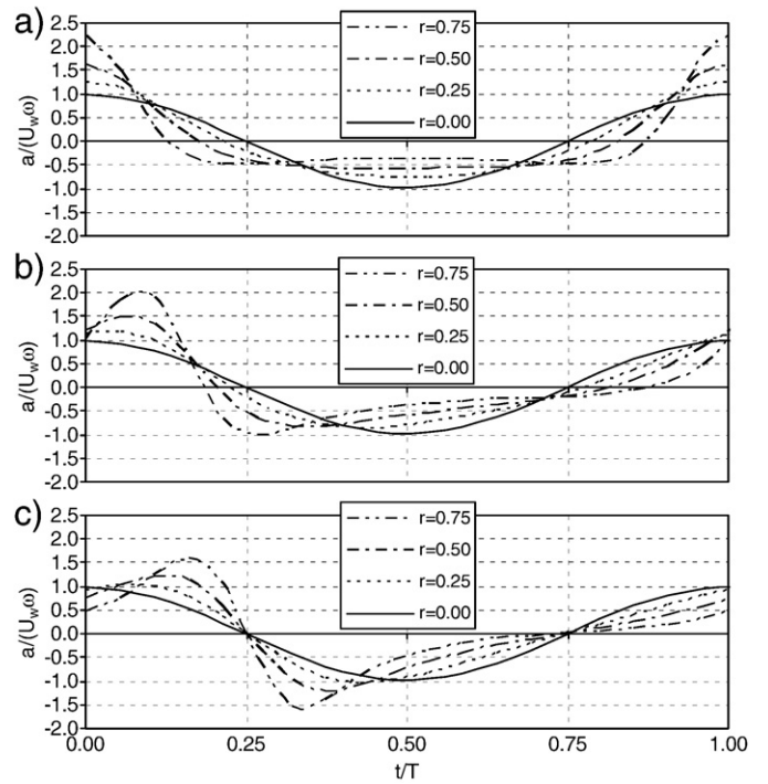
Fig. 2. Time varying orbital acceleration for different values of index of skewness r and \phi : a) \phi = 0 ; b) \phi = -\pi/4 ; c) \phi = -\pi/2 .
