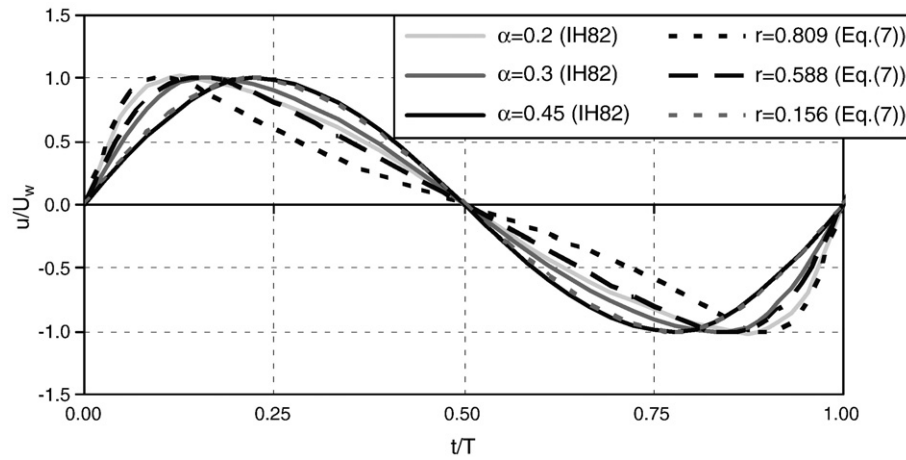
Fig. 8. Time varying orbital velocities: comparison between IH82 theory (—) and present formulation (---) for the sawtooth wave velocity profile ( \phi=0 ) and three values of the skewness index r .
