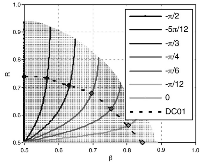
Fig. 10. Domain of solutions ( \beta , R ) for Eq. (7) (shaded area) and for DC01 (dashed line).
