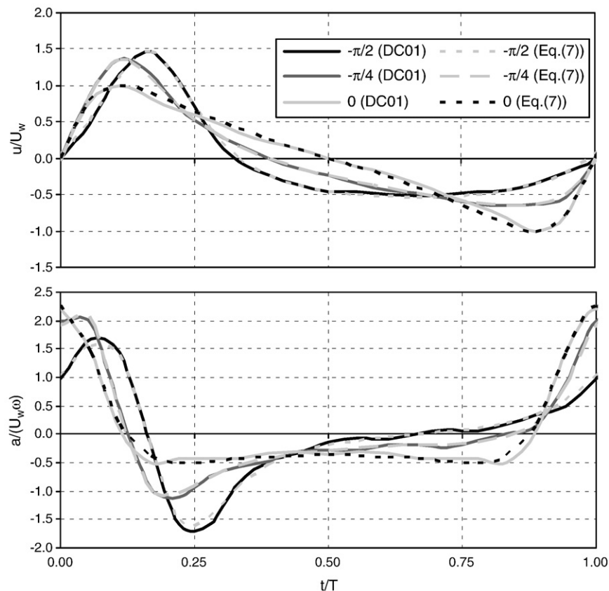
Fig. 9. Time varying orbital velocity and acceleration: comparison between DC01 theory (—) and Eq. (7) (---) for different \phi values.
