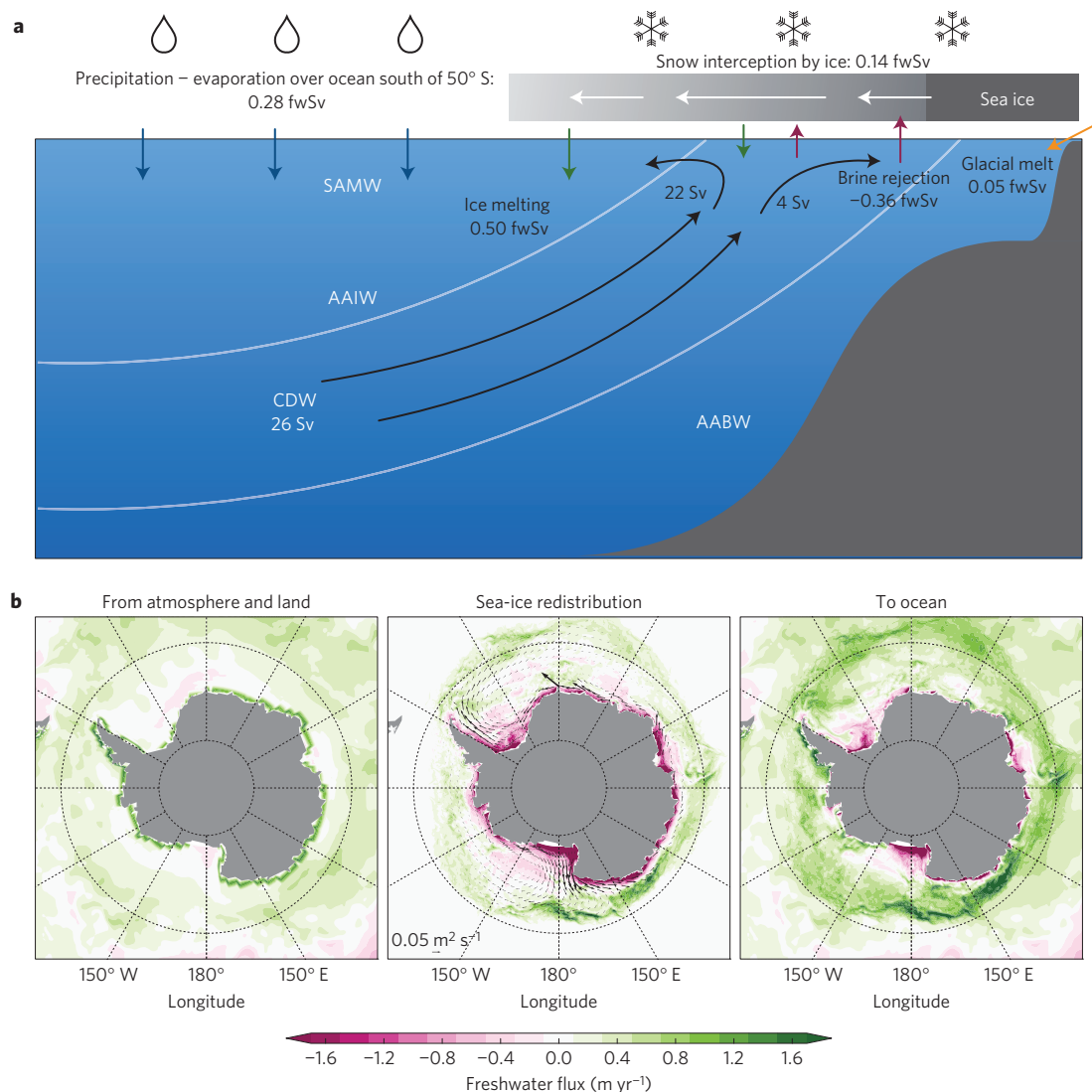
Figure 1 | Surface freshwater exchange in the SOSE. a , Schematic depicting the various bulk contributions to the freshwater exchange at the ocean surface south of 50° S (positive downward). Net fluxes are given in units of freshwater sverdrups 11 : 1 fwSv = 10 6 m -3 freshwater s -1 ≈ 3.15 × 10 4 Gt freshwater per year. For reference, 1 fwSv ≈ 1.9 mm d -1 of rainfall distributed over the region. b , Annual mean freshwater fluxes for the period 2005–2011. The left panel shows the flux leaving the atmosphere and land, and the right panel shows the flux entering the ocean. The centre panel shows the sea-ice redistribution flux (the difference between the two), with arrows indicating the lateral sea-ice thickness transport.
