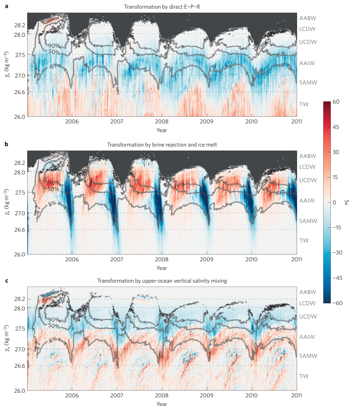
Figure 3 | Time series of freshwater transformation over the six-year state estimate, as a function of time (x axis) and neutral density \gamma_n (y axis).
