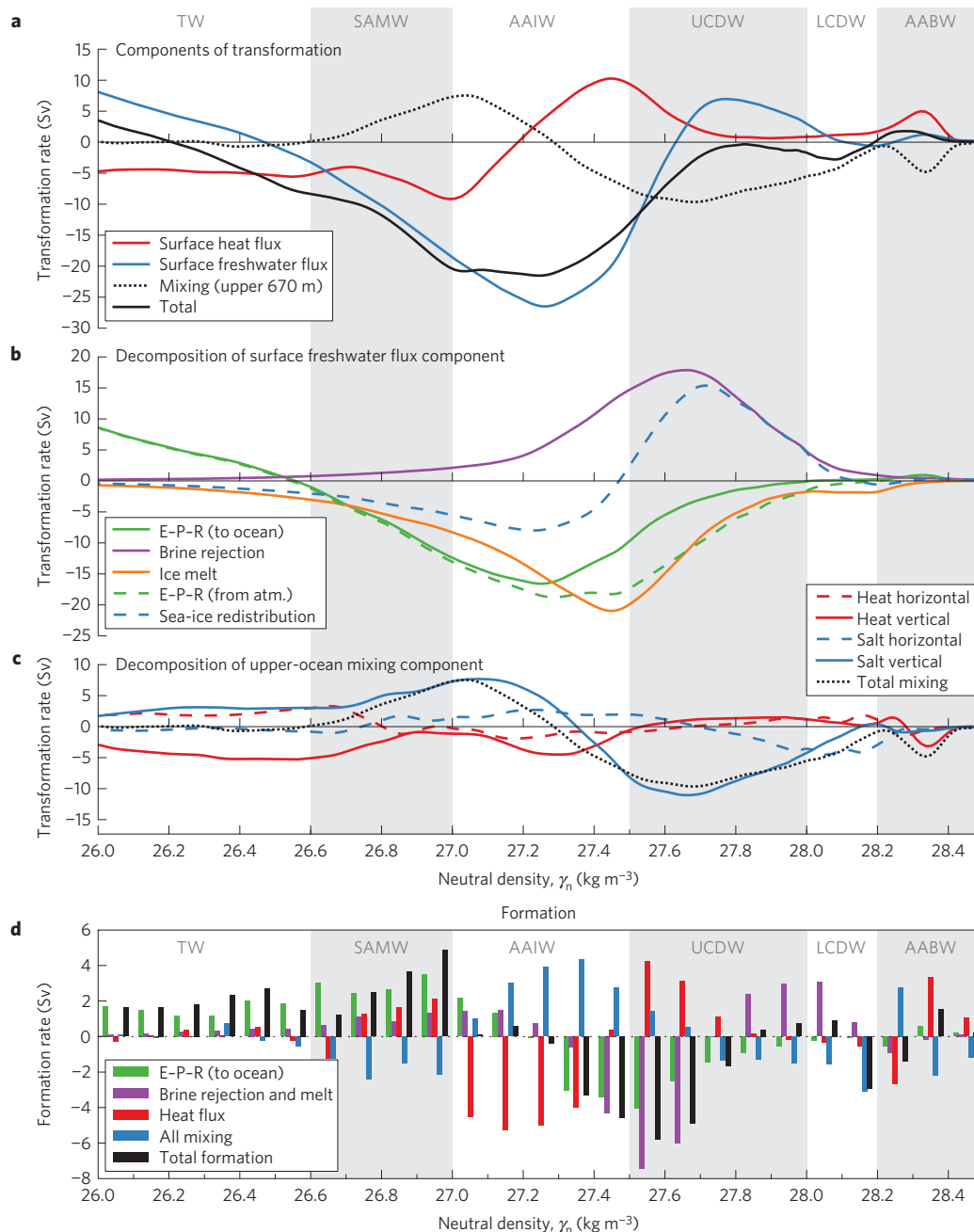
Figure 2 | Components of water-mass transformation and formation in SOSE in neutral density ( \gamma_n ) coordinates. The total transformation rate represents the net volume flux (in sverdrups, 1 \text{ Sv} = 10^6 \text{ m}^3 \text{ s}^{-1} ) across an isopycnal surface. a , Total water-mass transformation (black) decomposed into contributions from surface heat flux (red), surface freshwater flux (blue), and upper-ocean mixing (dotted black). b , Decomposition of the surface-freshwater-flux-driven transformation into contributions from direct exchange with the atmosphere, land and terrestrial ice (evaporation, precipitation and runoff/glacial ice melt; green), brine rejection from freezing sea ice (purple), and freshwater from melting ice (orange); the three solid lines in b sum to give the blue line in a . An alternative decomposition of the freshwater-driven transformation into the sum of the potential transformation that would have occurred due to the atmospheric freshwater flux (dashed green) and the redistribution of freshwater by the sea ice (dashed blue). atm., atmosphere. c , Decomposition of mixing-induced transformation into contributions from vertical (solid) and horizontal/isopycnal (dashed) mixing of heat (red) and salt (blue) in the upper 670 m (a depth that encompasses most of the seasonal mixed layer). The black dotted line represents total mixing. d , Formation rates, summed in 0.1 \text{ kg m}^{-3} neutral density bins, representing the convergence or divergence of water-mass transformation in the upper ocean. The total formation (black) is the sum of the coloured bars, which represent direct exchange with the atmosphere, land and terrestrial ice (evaporation, precipitation and runoff/glacial ice melt; green), sea-ice brine rejection and melt (purple), surface heat flux (red), and mixing (blue). The large-scale water masses are abbreviated as thermocline water (TW), Subantarctic Mode Water (SAMW), Antarctic Intermediate Water (AAIW), Upper Circumpolar Deep Water (UCDW), Lower Circumpolar Deep Water (LCDW), and Antarctic Bottom Water (AABW).
