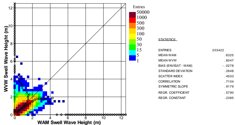
Fig. 6. Global comparison between ASAR Level 2 and ECMWF model swell significant wave height during the period from 11 April to 31 August 2005.
