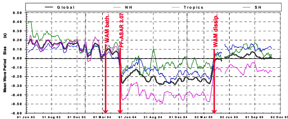
Fig. 3. Time series of mean wave period bias between ASAR Level 1b inverted product and wave model.
