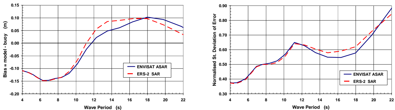
Fig. 9. ASAR assimilation impact on wave spectrum according to buoy data around Hawaii in terms of equivalent 2-s significant wave height (1-30 April 2005)
