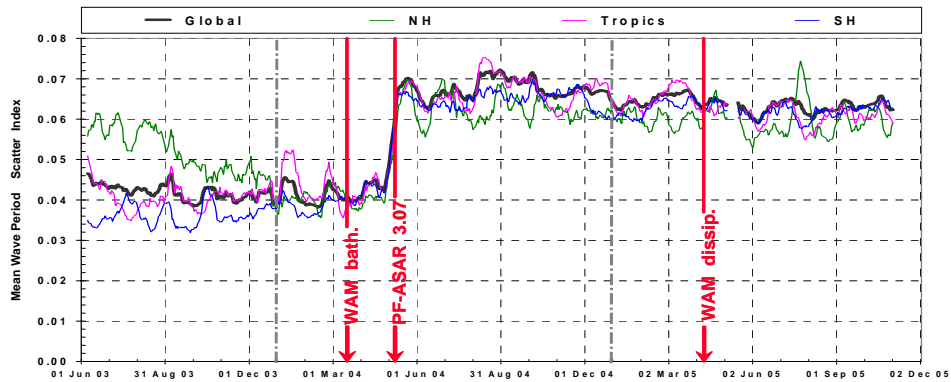
Fig. 4. Time series of mean wave period scatter index between ASAR Level 1b inverted product and wave model.
