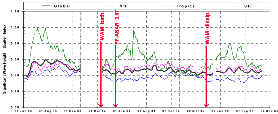
Fig. 8. Time series of swell significant wave height scatter index between ASAR Level 2 product and wave model.
