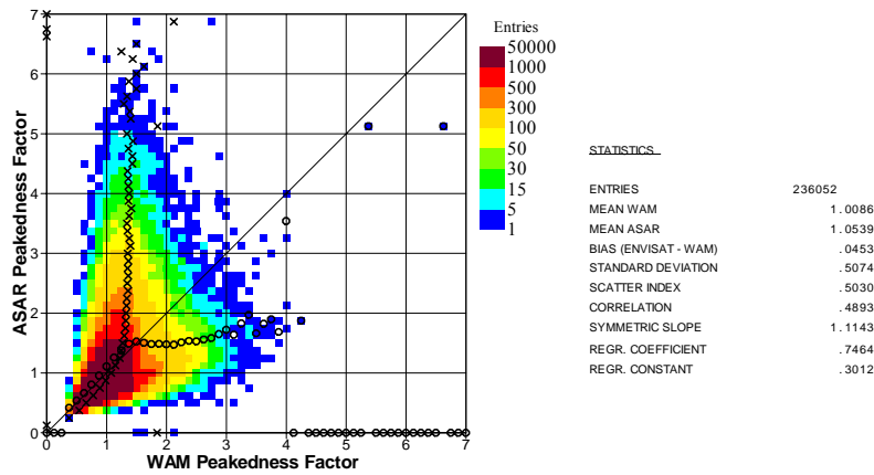
Fig. 2. Global comparison between inverted ASAR Level 1b and ECMWF model wave spectral peakedness factor of Goda during the period from 11 April to 31 August 2005.
