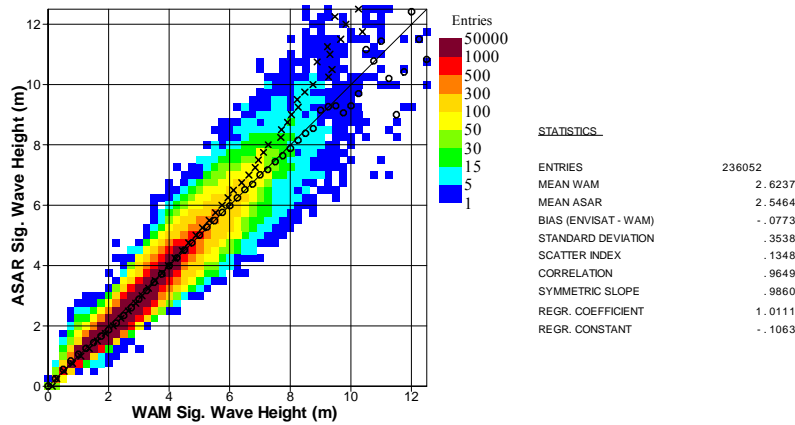
Fig. 1. Global comparison between inverted ASAR Level 1b and ECMWF model significant wave height during the period from 11 April to 31 August 2005.
