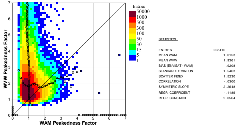
Fig. 7. Global comparison between ASAR Level 2 and ECMWF model swell wave spectral peakedness factor of Goda during the period from 11 April to 31 August 2005.
