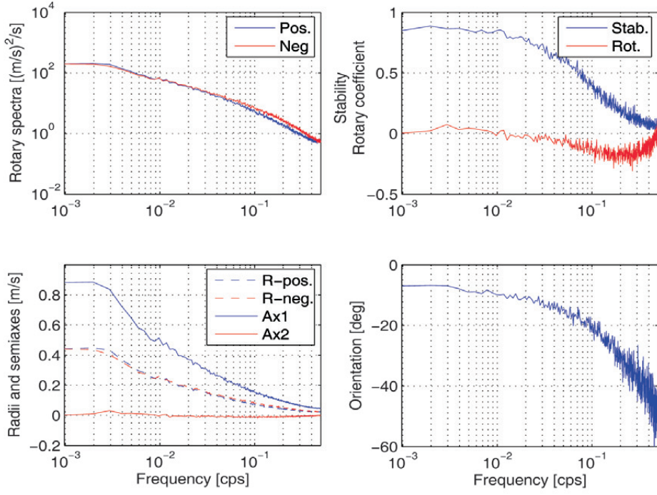
Figure 3. Spectra of rotary components and related parameters for the whole bora episode considered.
