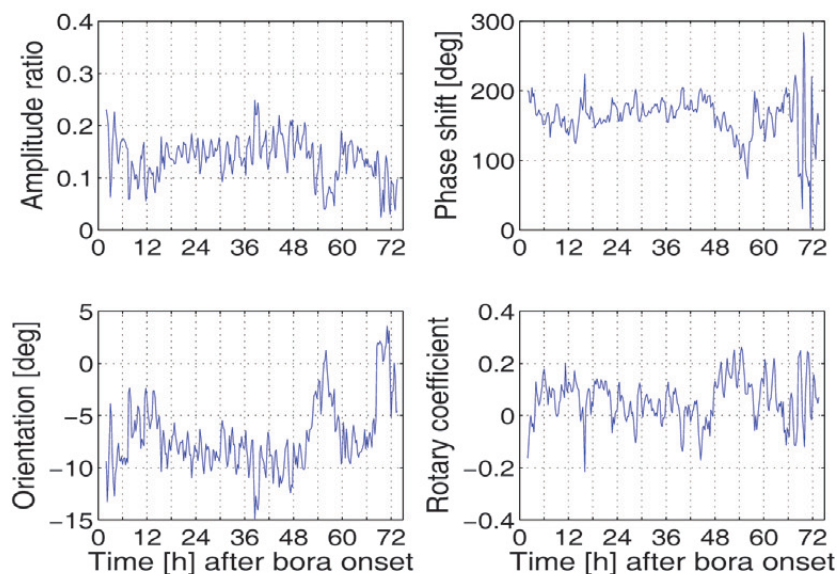
Figure 5. Results of cross-spectral analysis of the horizontal and vertical wind components (up) and of rotary spectral analysis (down), for the 5.7 min period.
