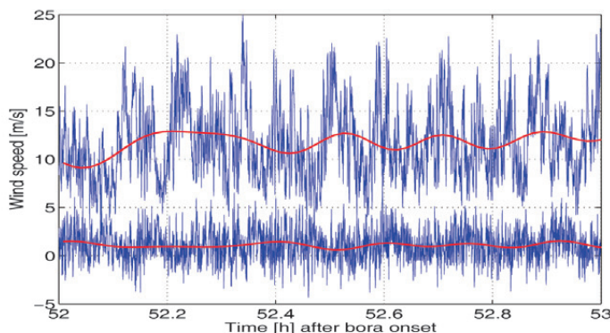
Figure 1. Horizontal (up) and vertical (down) wind components: 1 s and 10 min values.
